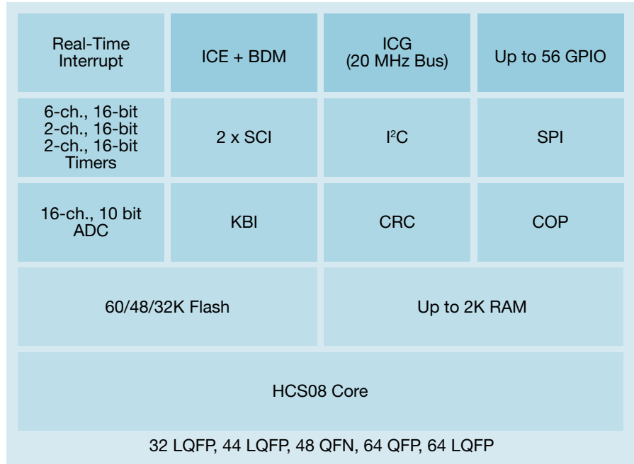
AC60 Block Diagram
