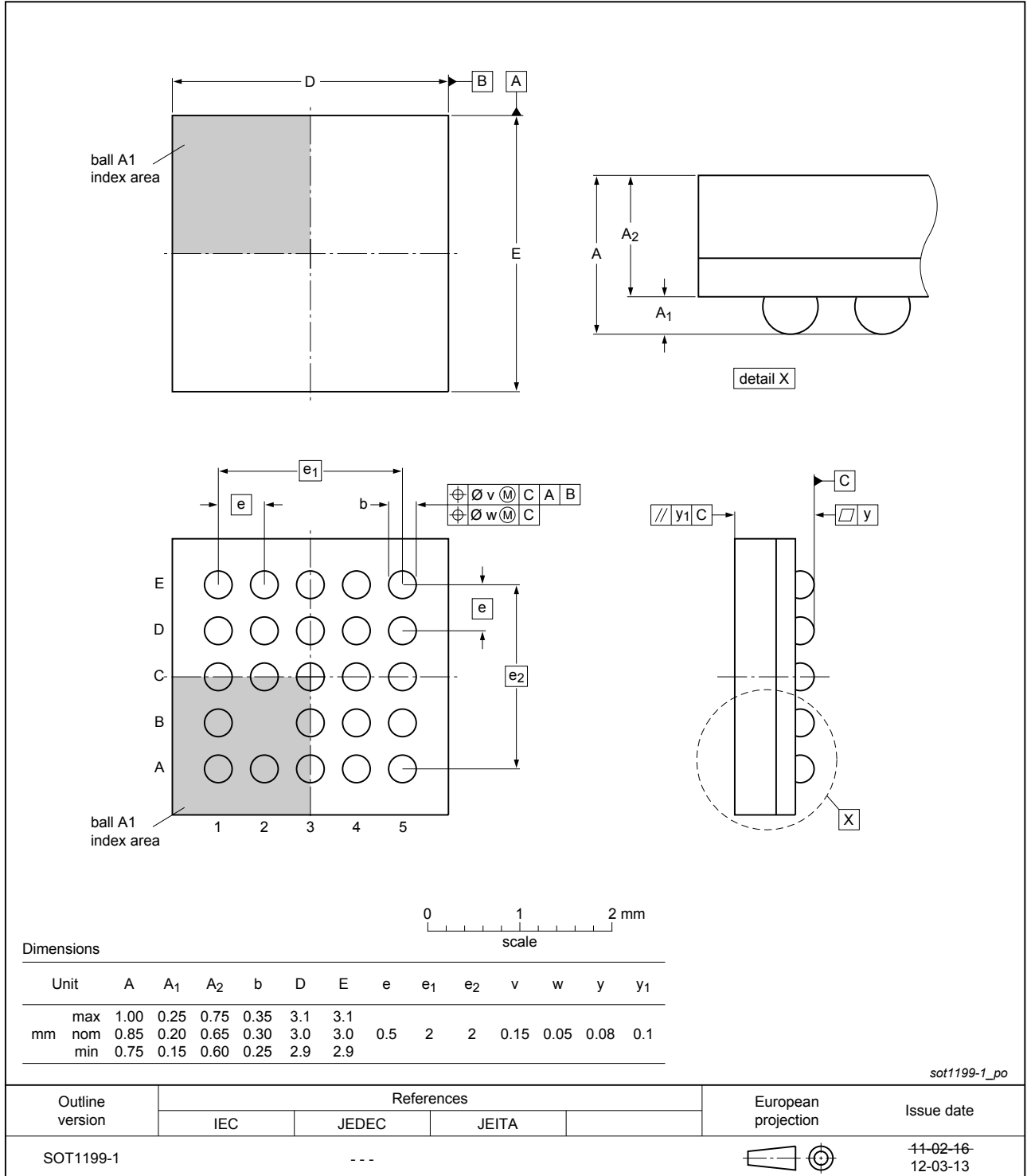
Fig. 1. Package outline VFBGA24 (SOT1199-1)
