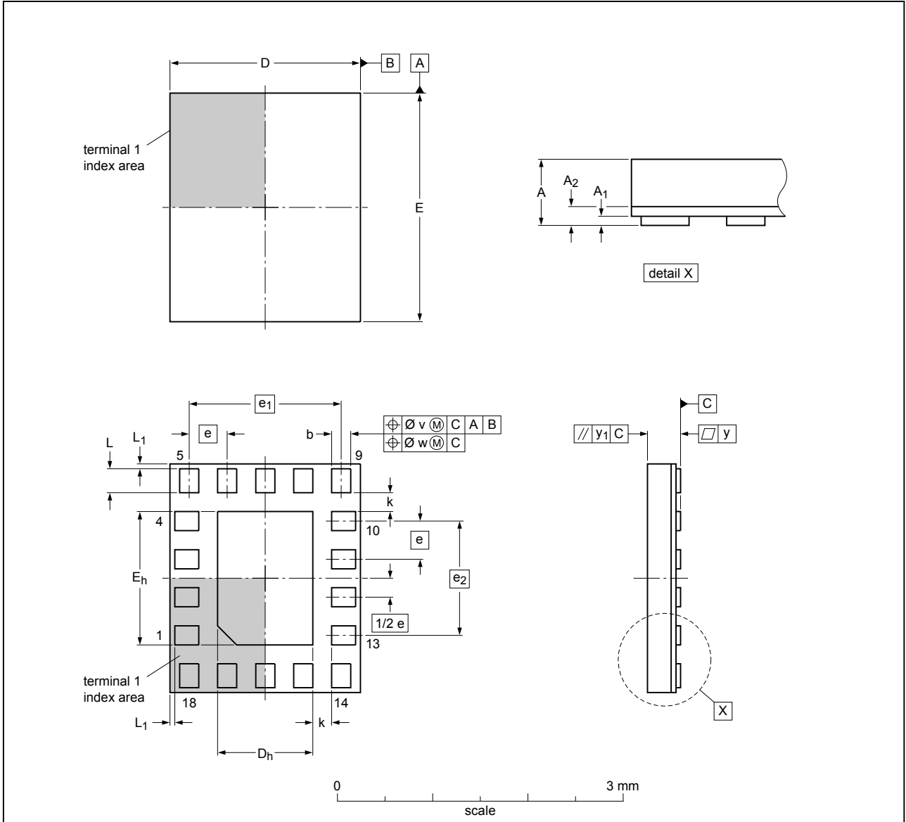
DHX2QFN18: plastic dual in-line compatible thermal enhanced super-thin quad flat package; no leads; 18 terminals; body 2.4 x 2.0 x 0.35 mm
