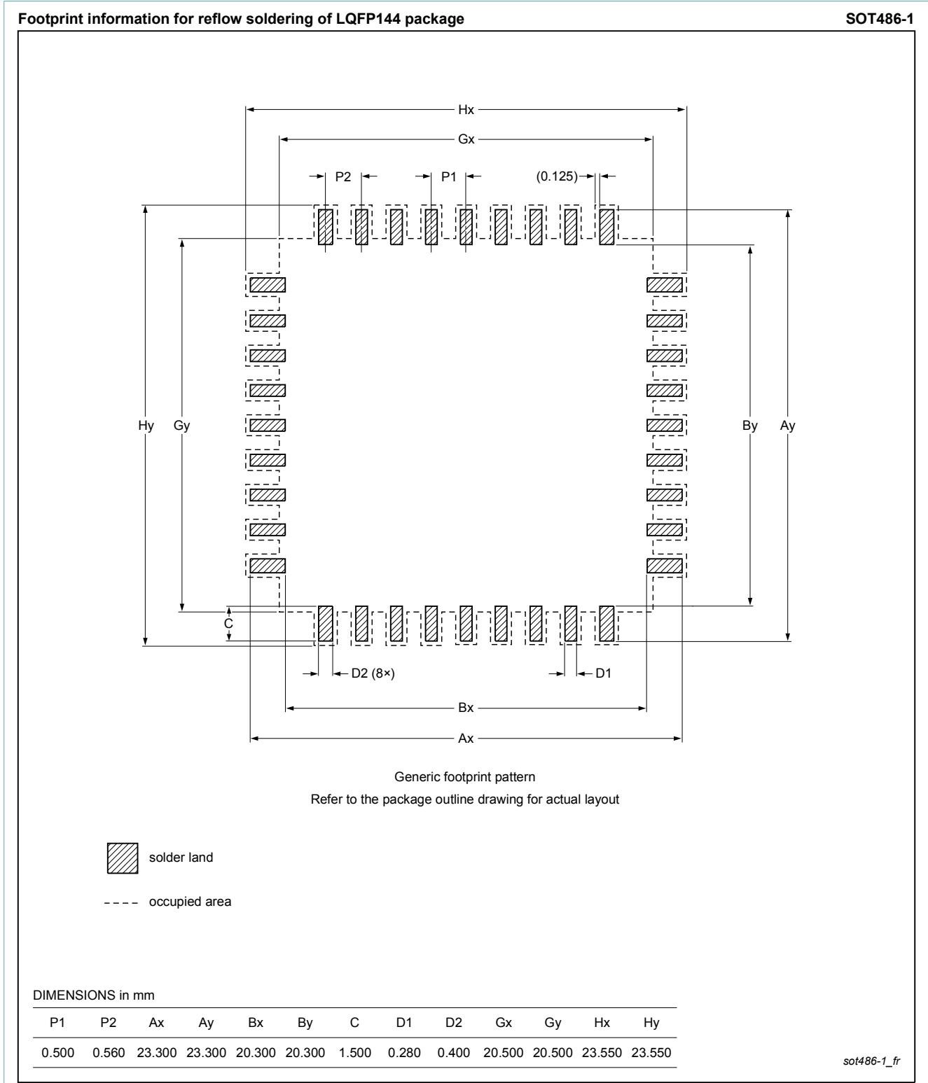
Fig. 2. Reflow soldering footprint for LQFP144 (SOT486-1)
