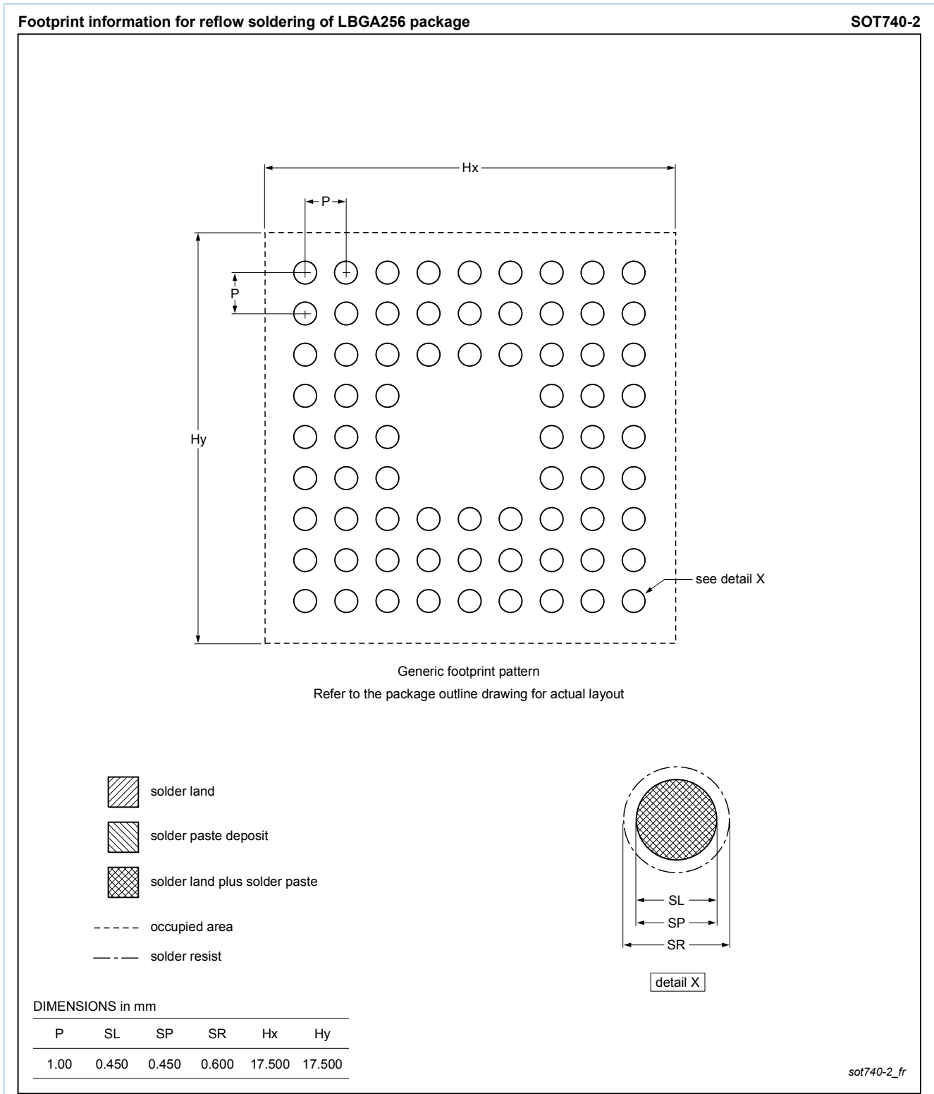
Fig. 2. Reflow soldering footprint for LBG256 (SOT740-2)
