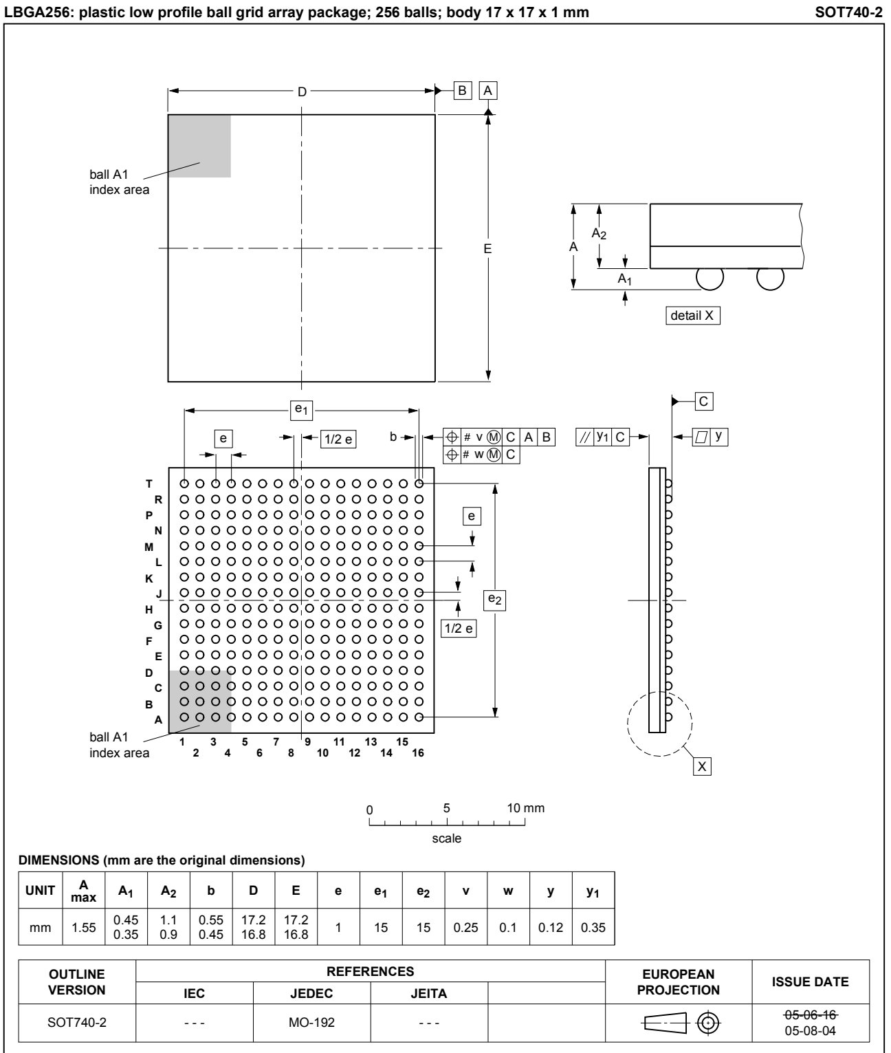
Fig. 1. Package outline LPGA256 (SOT740-2)
