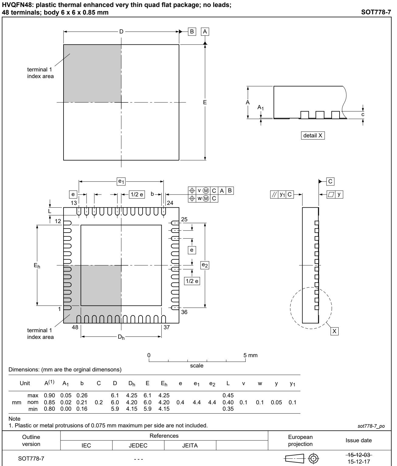
Fig. 1. Package outline HVQFN48 (SOT778-7)
