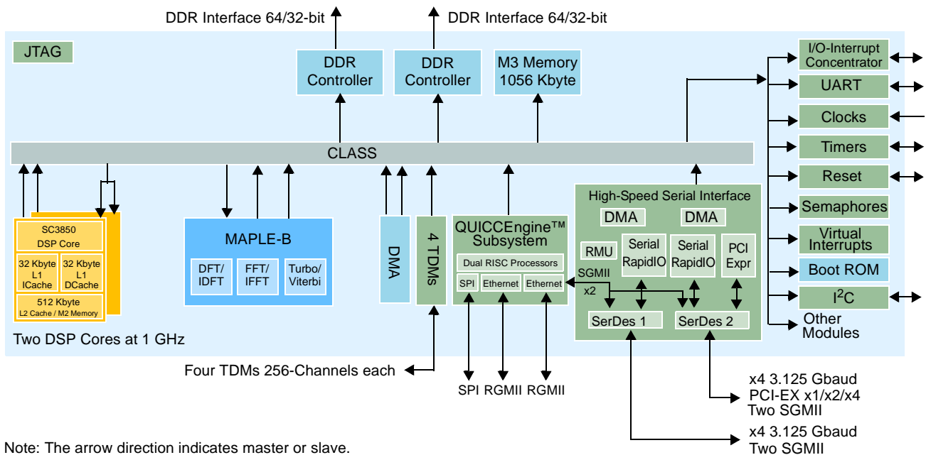
Figure 1-1. MSC8152 Block Diagram
