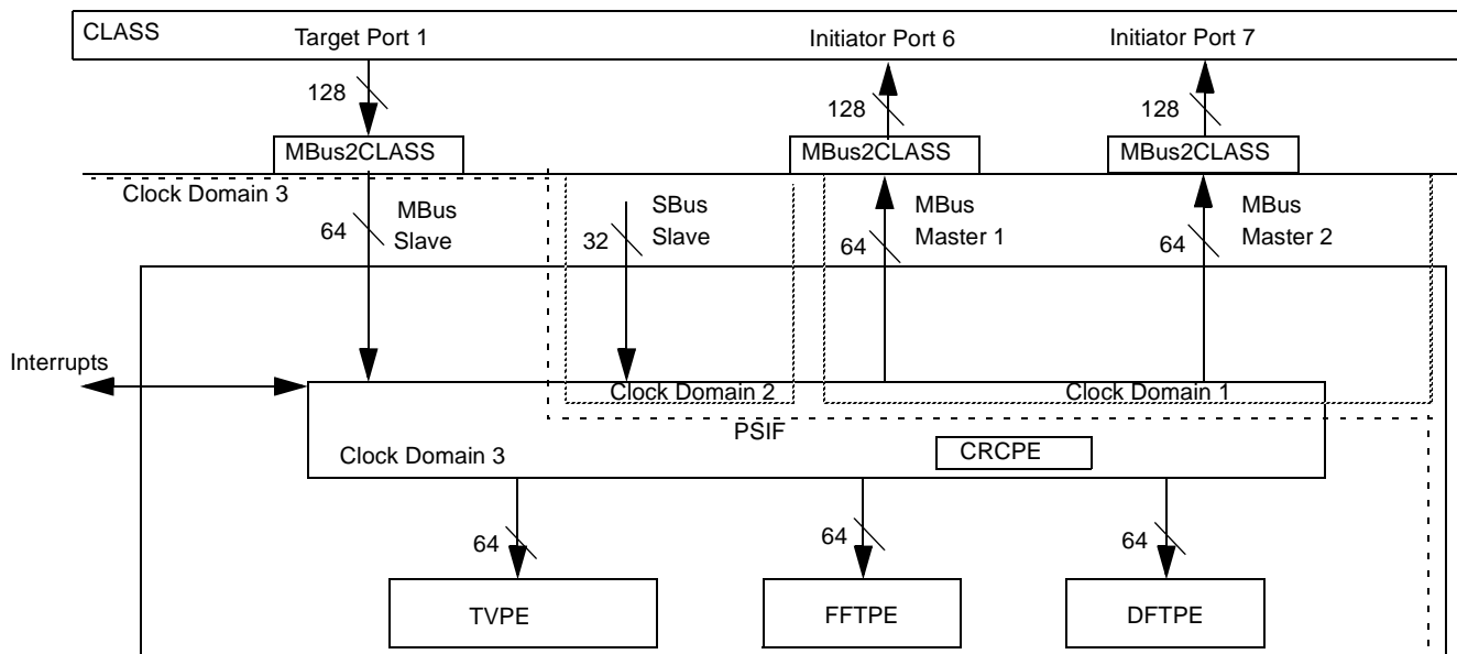
Figure 26-1. MAPLE-B Overview
