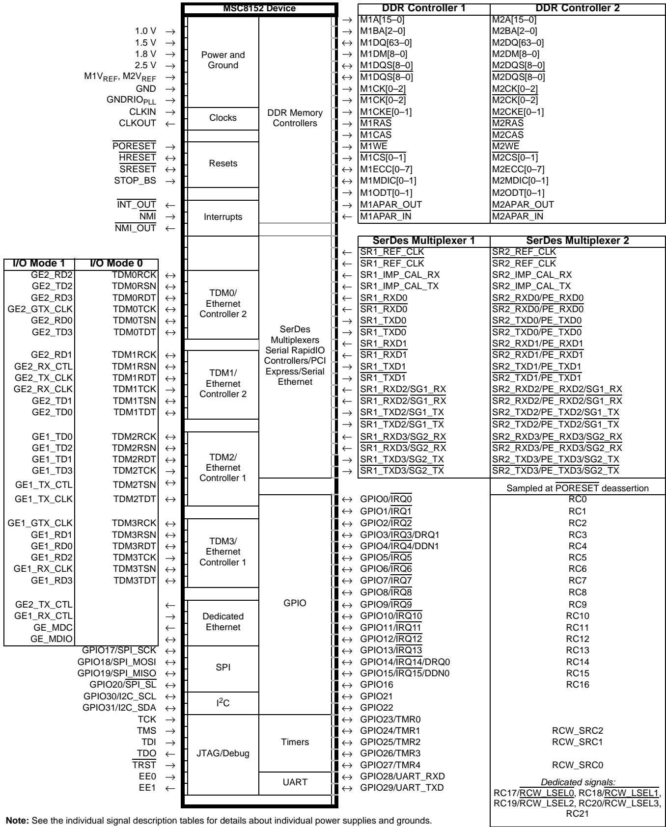
Figure 3-1. MSC8152 External Signals
