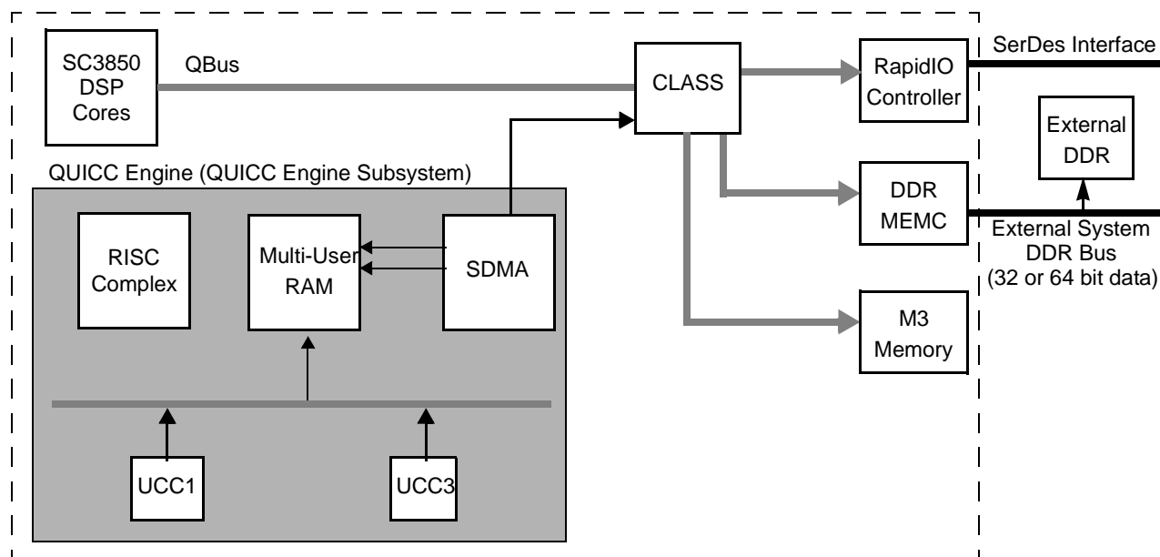
Figure 18-4. MSC8152 Data Paths
