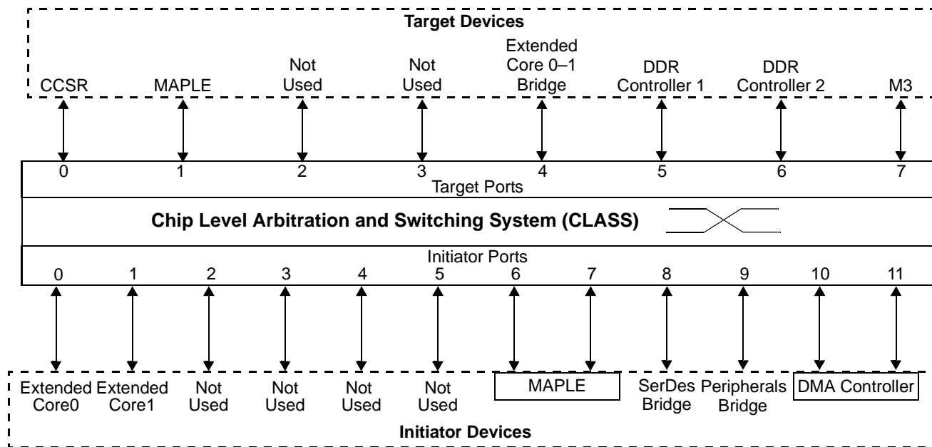
Figure 4-1. CLASS Initiators and Targets in the MSC8152 Device
