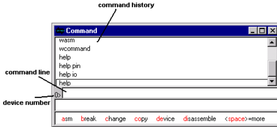
Figure 11-2. Displaying the Command Window
