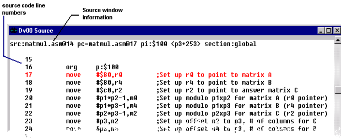
Figure 11-5. Displaying the Source Window
