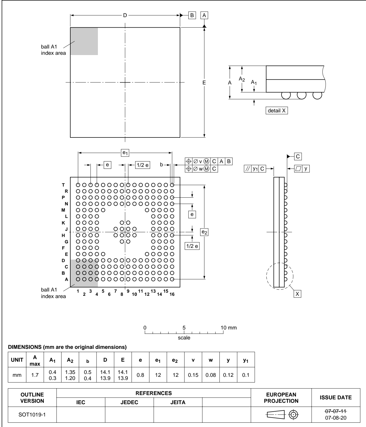
LFBGA208: plastic low profile fine-pitch ball grid array package; 208 balls
