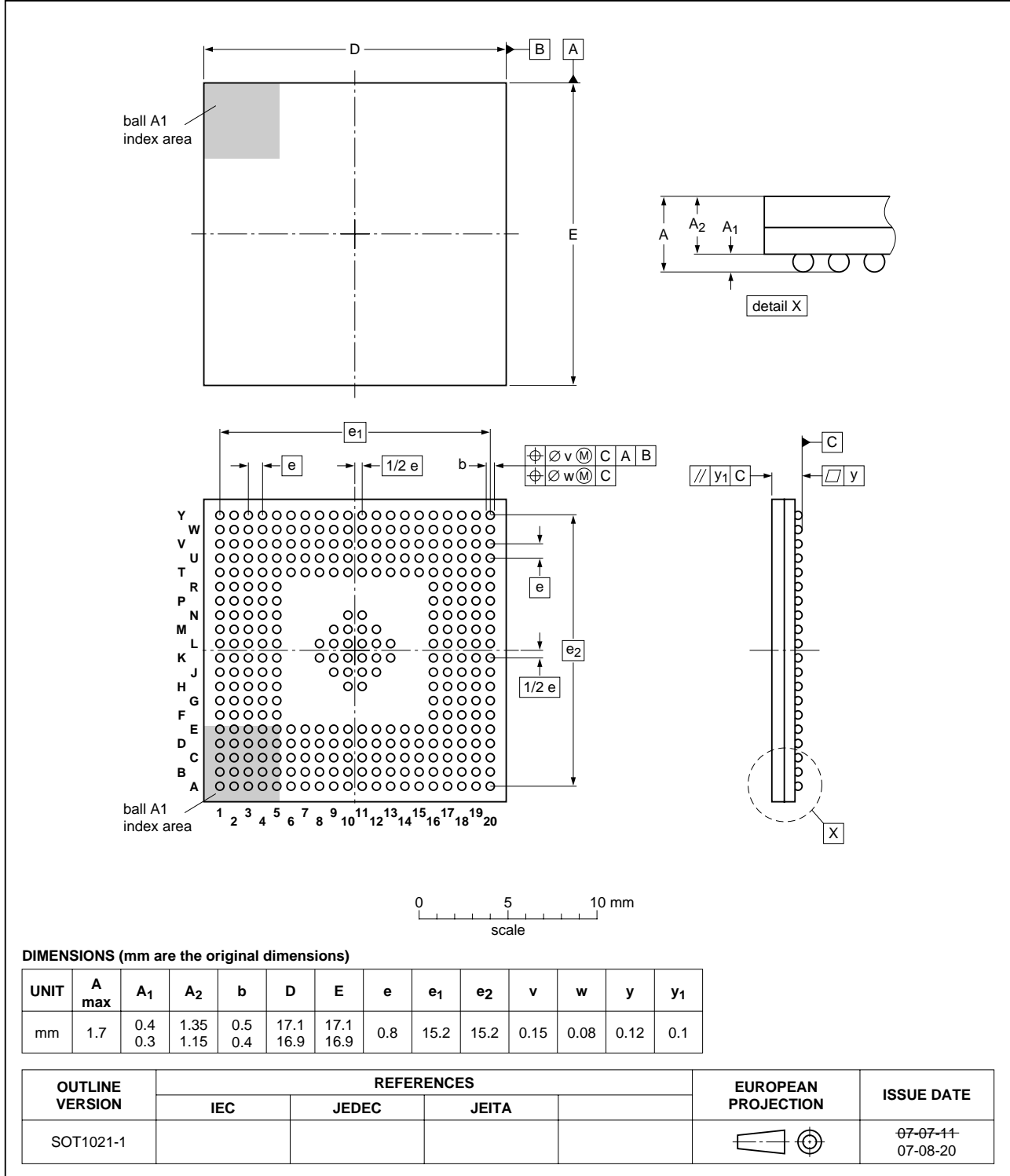
LFBGA324: plastic low profile fine-pitch ball grid array package; 324 balls
