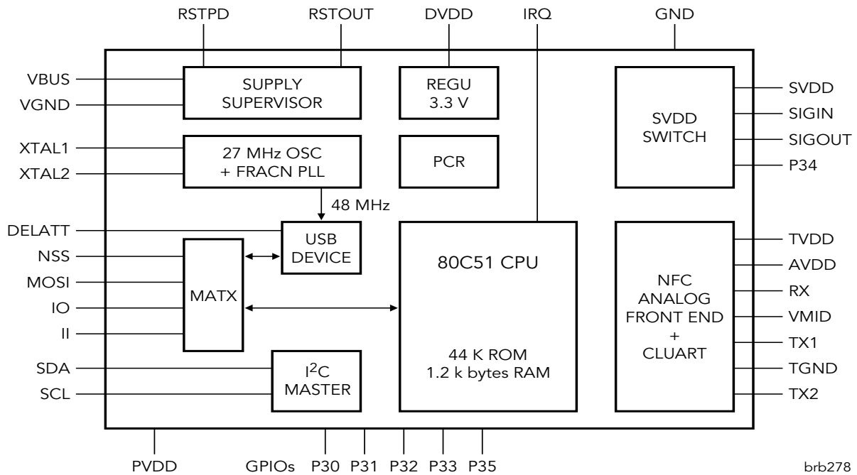
Block diagram
