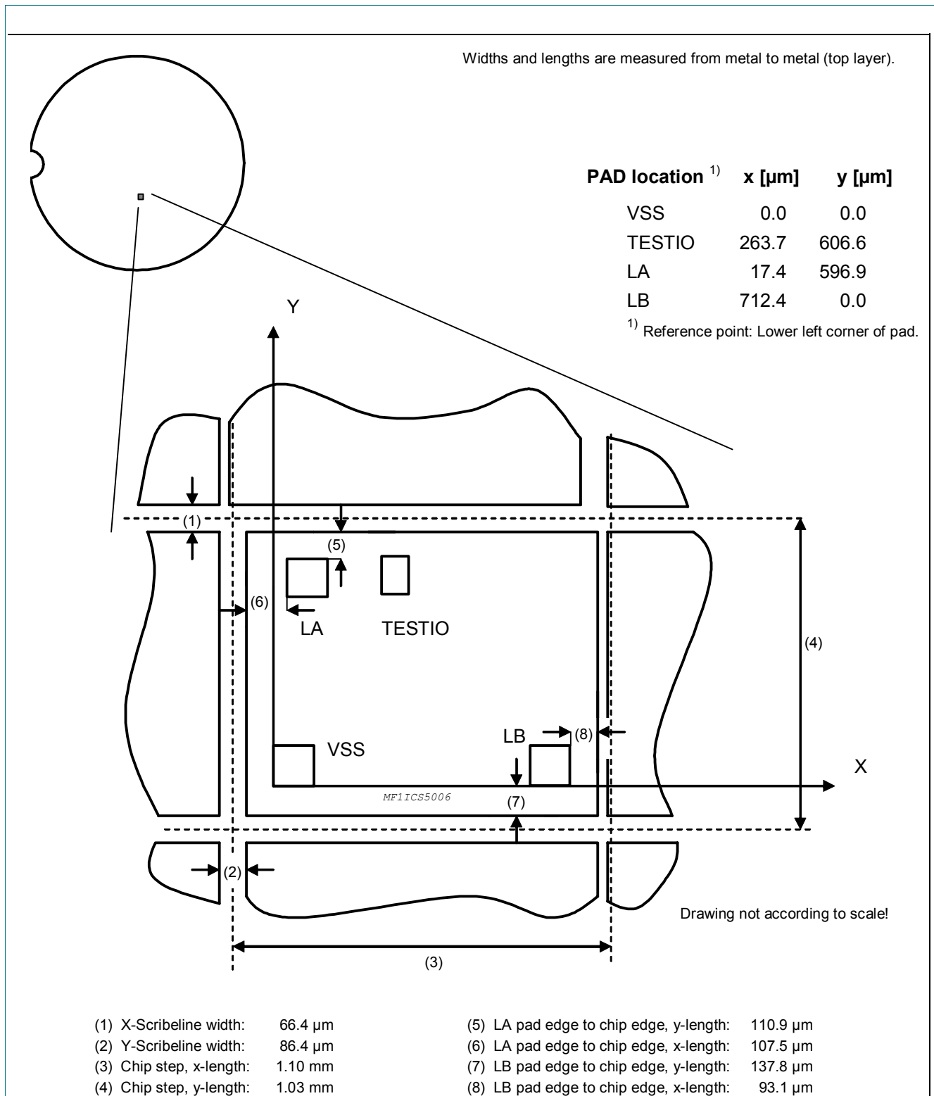
Fig 1. Chip orientation and bond pad locations
