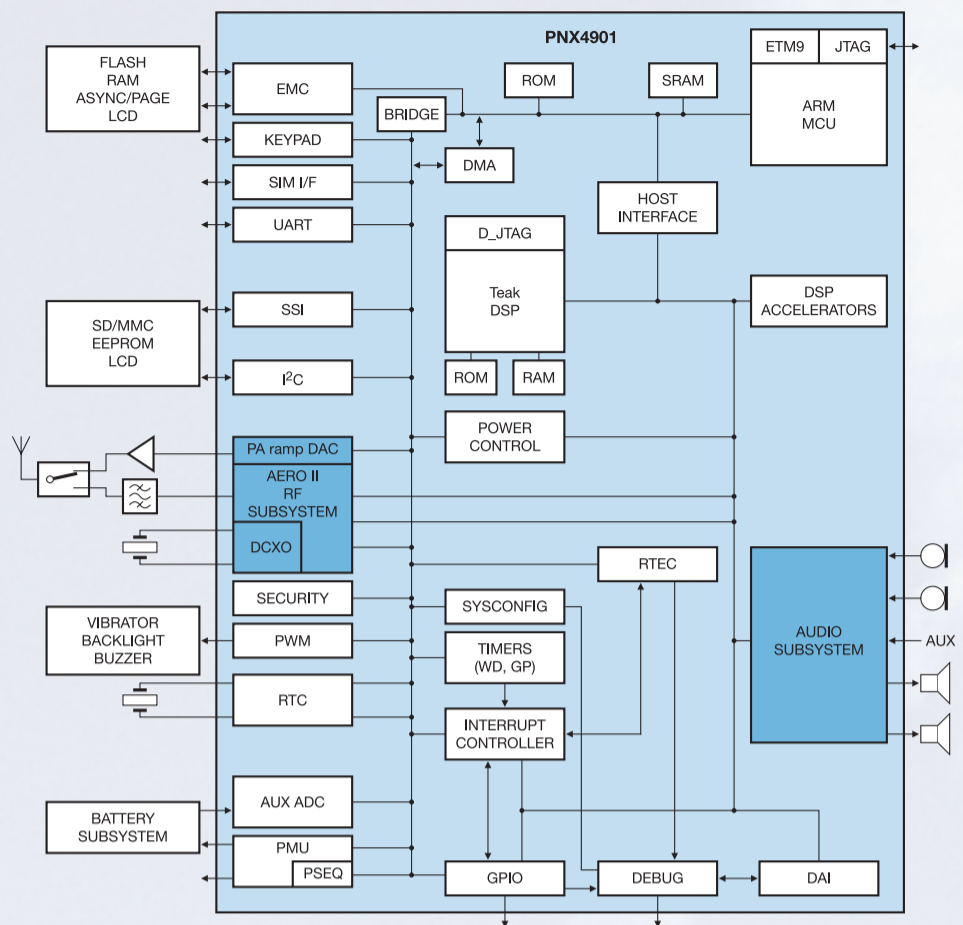
NXP single-chip GSM/GPRS ultra-low-cost solution PNX490x
