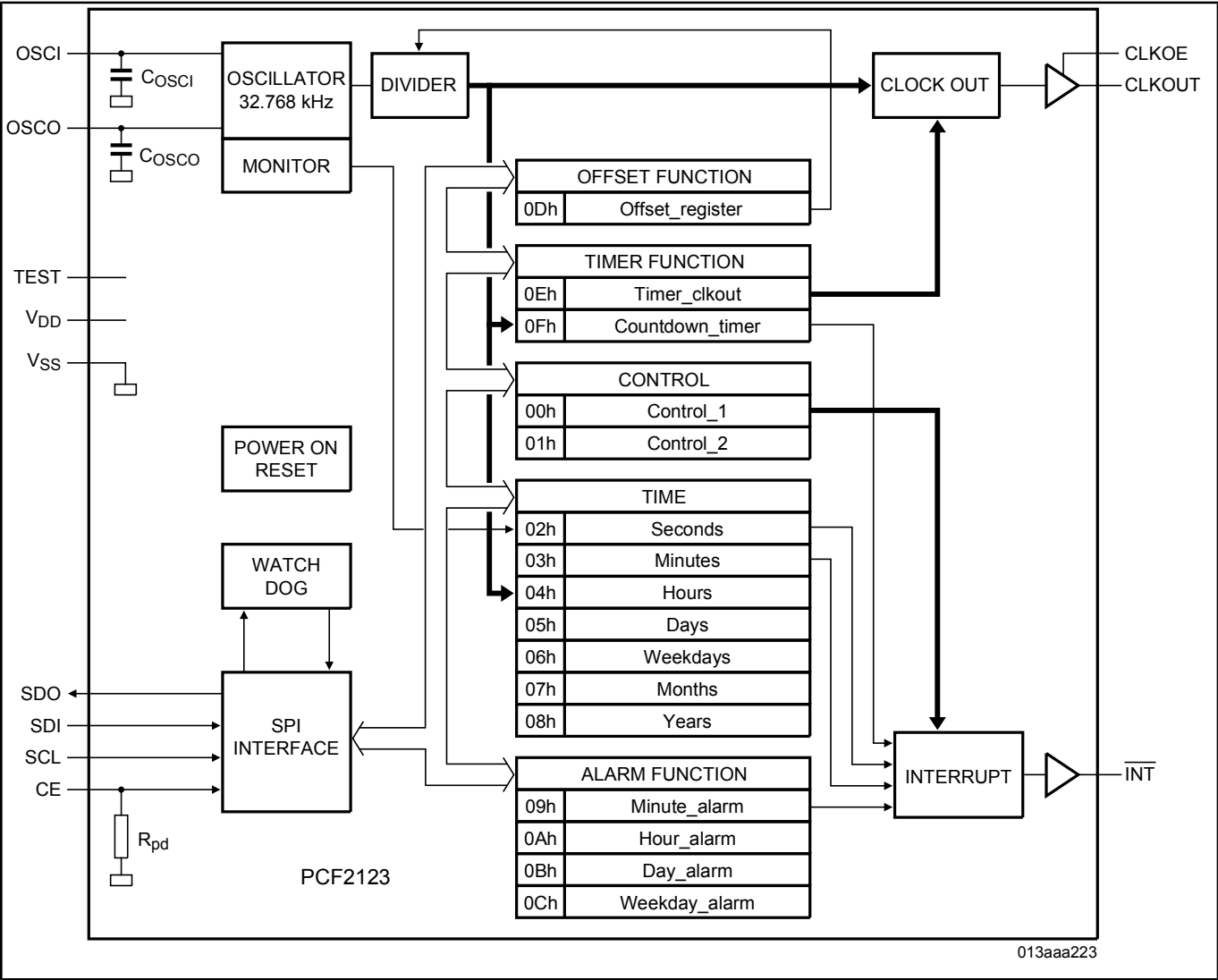
PCF2123 Block Diagram Block Diagram
