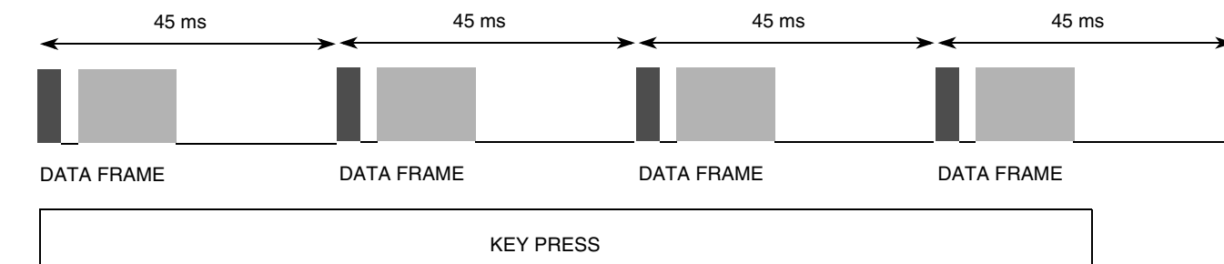
Figure 18. Pulse Width Protocol, Full Sequence Structure
