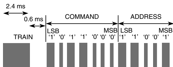
Figure 17. Pulse Width Protocol, Data Frame Structure
