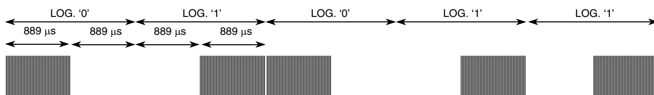
Figure 19. RC5 Protocol, Bit Encoding
