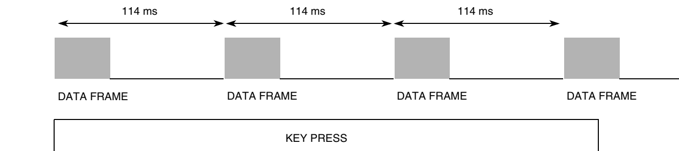
Figure 21. RC5 Protocol, Full Sequence Structure
