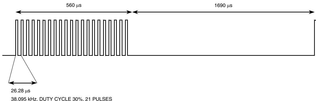
Figure 10. Example Waveform of Pulse Distance Encoded Bit
