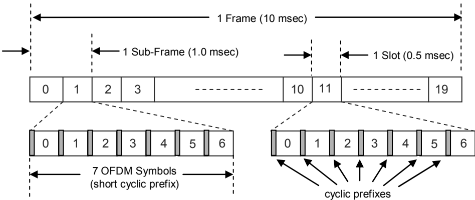
Figure 3.0.1-1 LTE Generic Frame Structure
