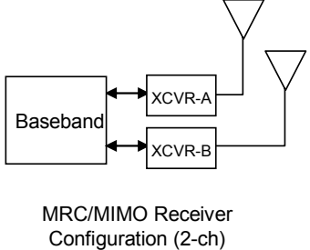
Figure 2.4-1a MRC/MIMO Operation Requires Multiple Transceivers
