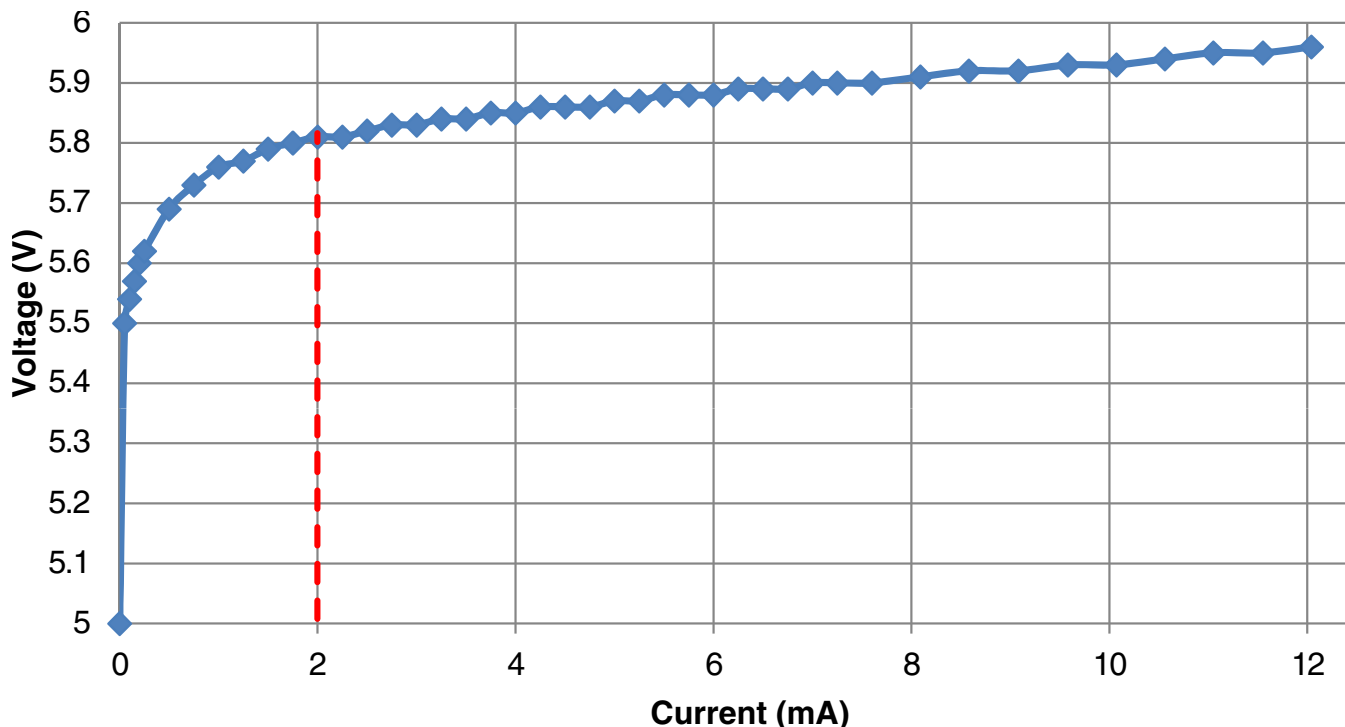
Figure 6. MPC5554 pin GPIO[203] digital pin injection current versus voltage, 25°C, V_{DDEH} = 5\text{V}
