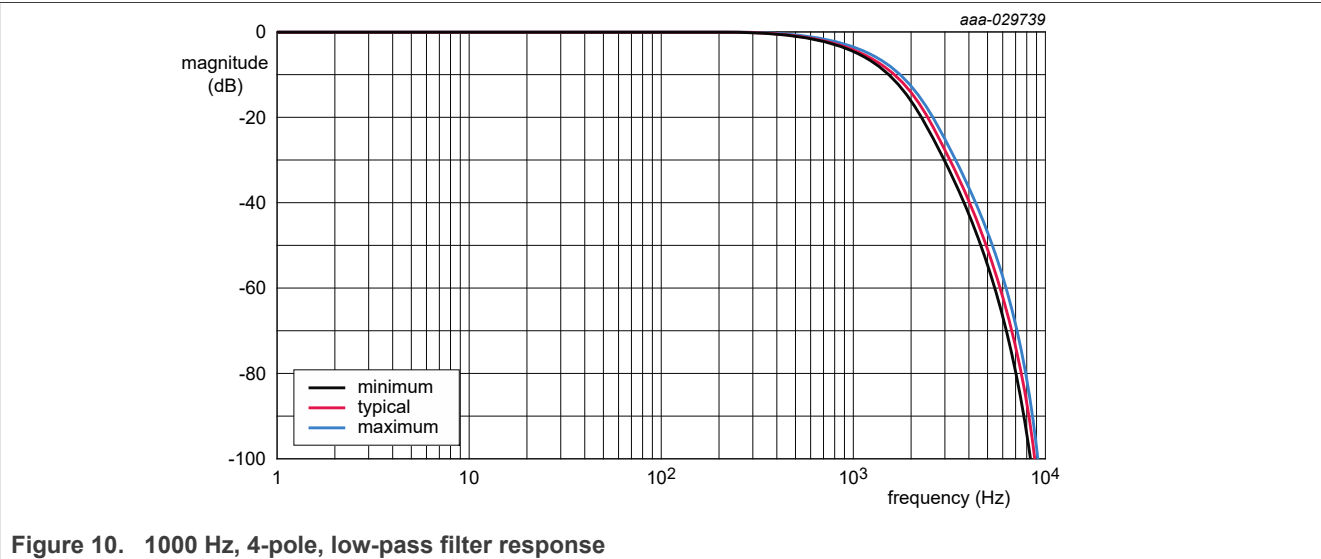
Figure 10. 1000 Hz, 4-pole, low-pass filter response
