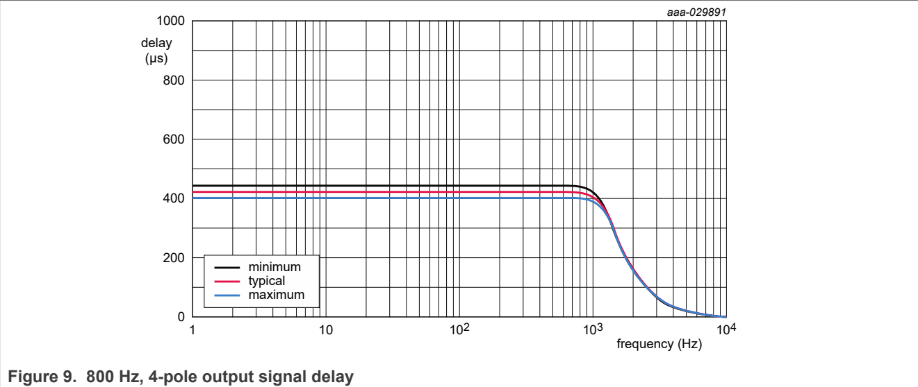
Figure 9. 800 Hz, 4-pole output signal delay
