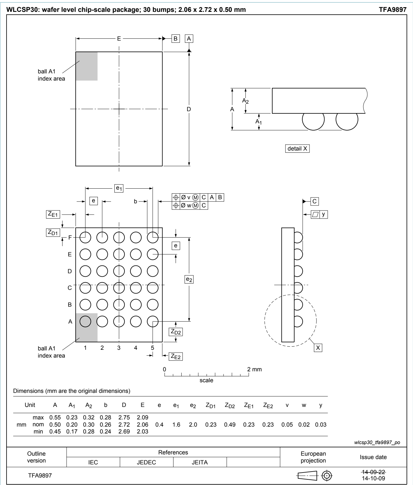
Fig. 1. Package outline WLCSP (OL-TFA9897)
