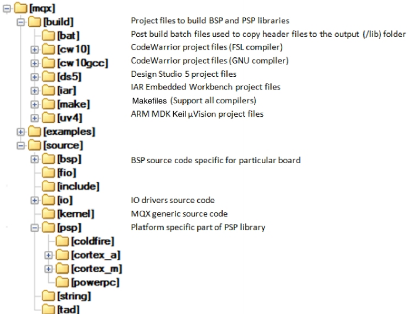
Figure 3. MQX PSP and BSP Directory Structure
