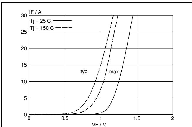
Fig.7. Typical and maximum forward characteristic
