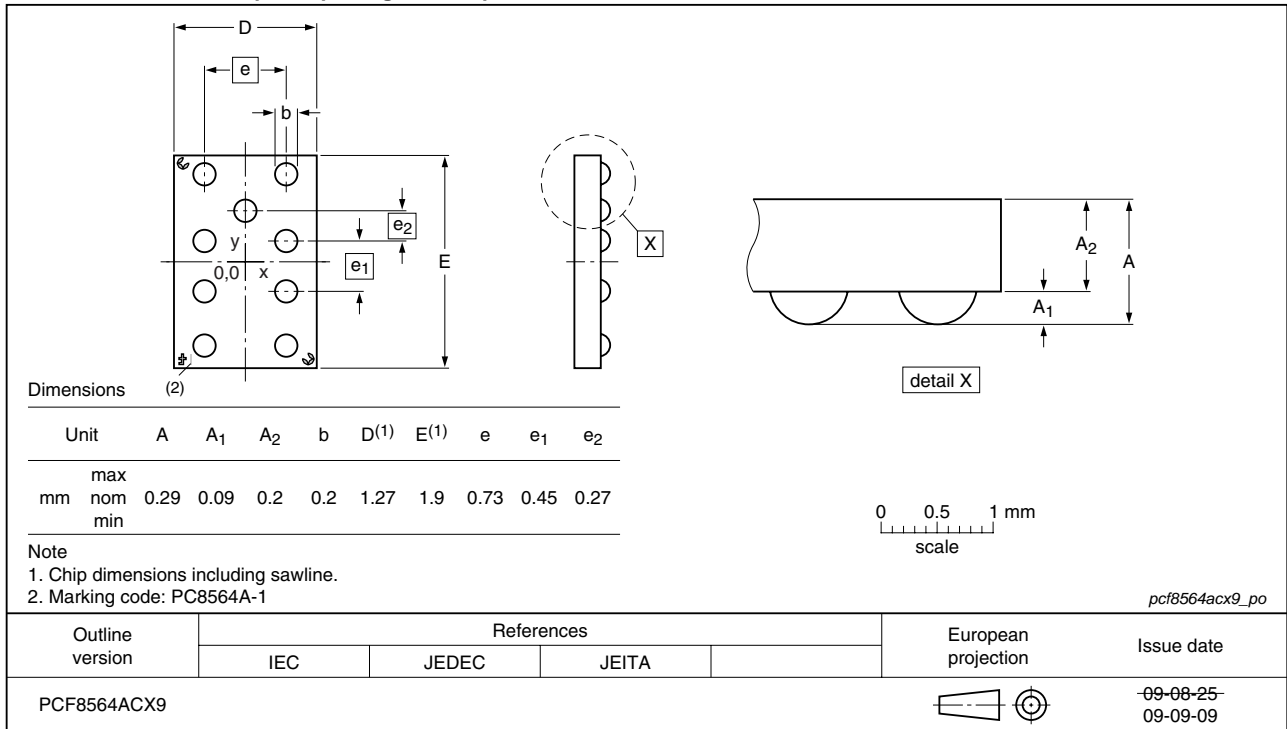
WLCSP9: wafer level chip-size package; 9 bumps; 1.27 x 1.9 x 0.29 mm
