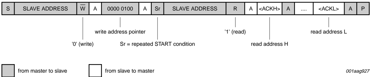
Fig 5. Host reads TDA9951 status register without setting address pointer (pointer was at 0 already)
