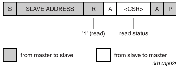
Fig 4. Host reads TDA9951 status register after setting address pointer
