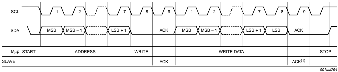
Fig 25. I 2 C-bus write
