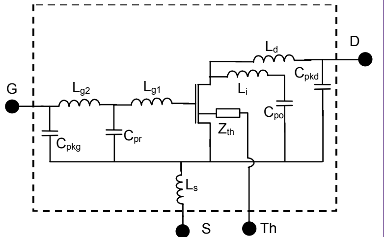
Fig 3. Schematic of the package model as in Fig 2.
