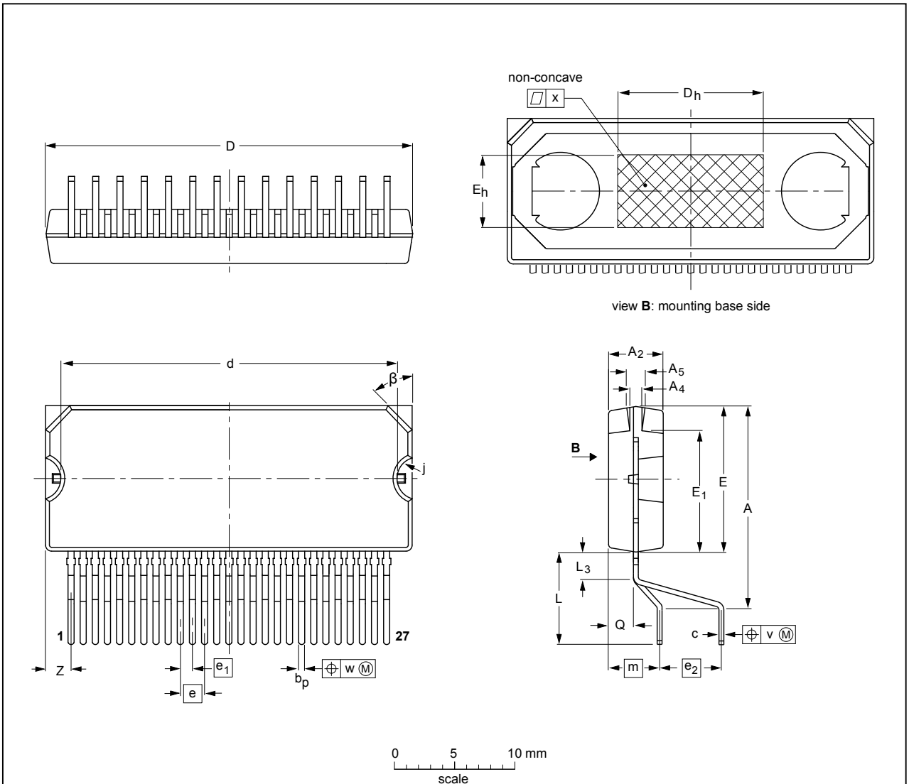
DBS27P: plastic DIL-bent-SIL power package; 27 leads (lead length 7.7 mm)
