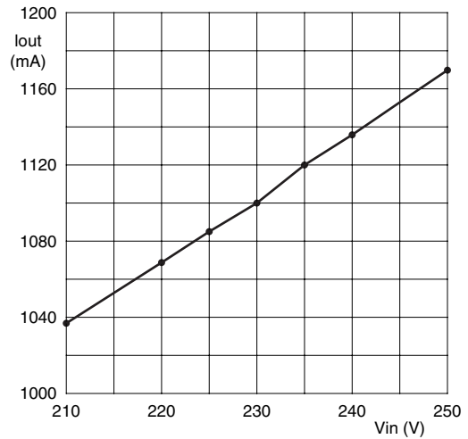
b. 230 V (AC) Input voltage dependency
