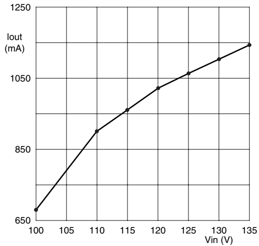
a. 120 V (AC) Input voltage dependency
