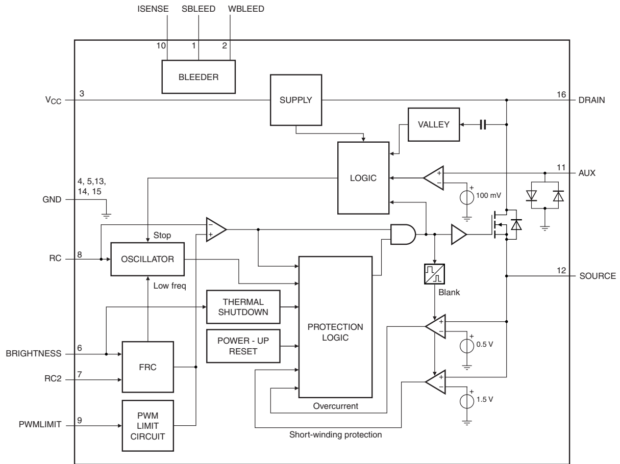
Fig 5. Block diagram SSL2102
