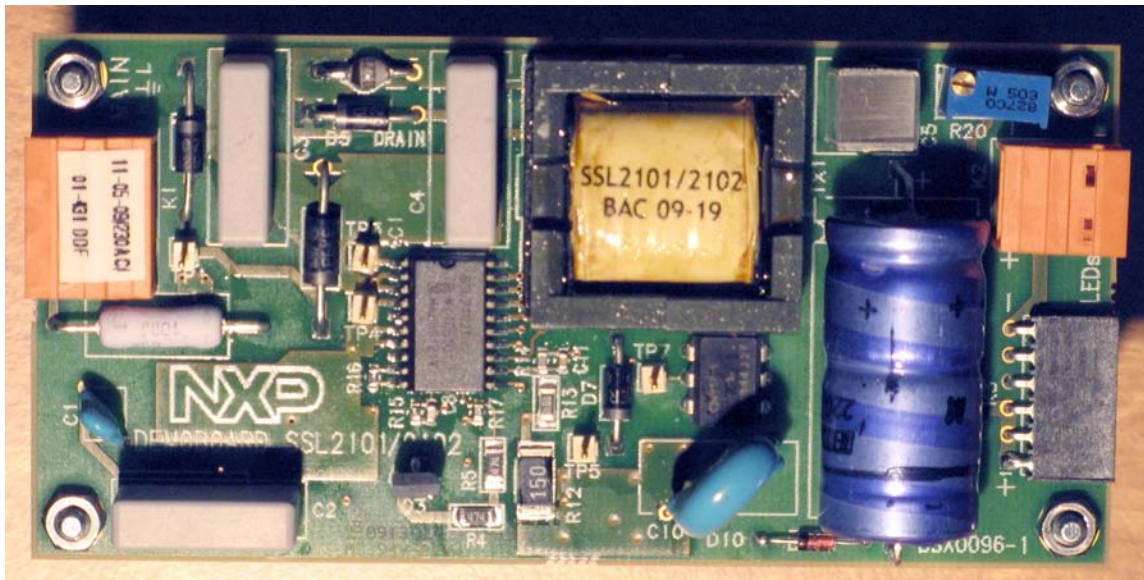
Fig 3. Demo board (top)
