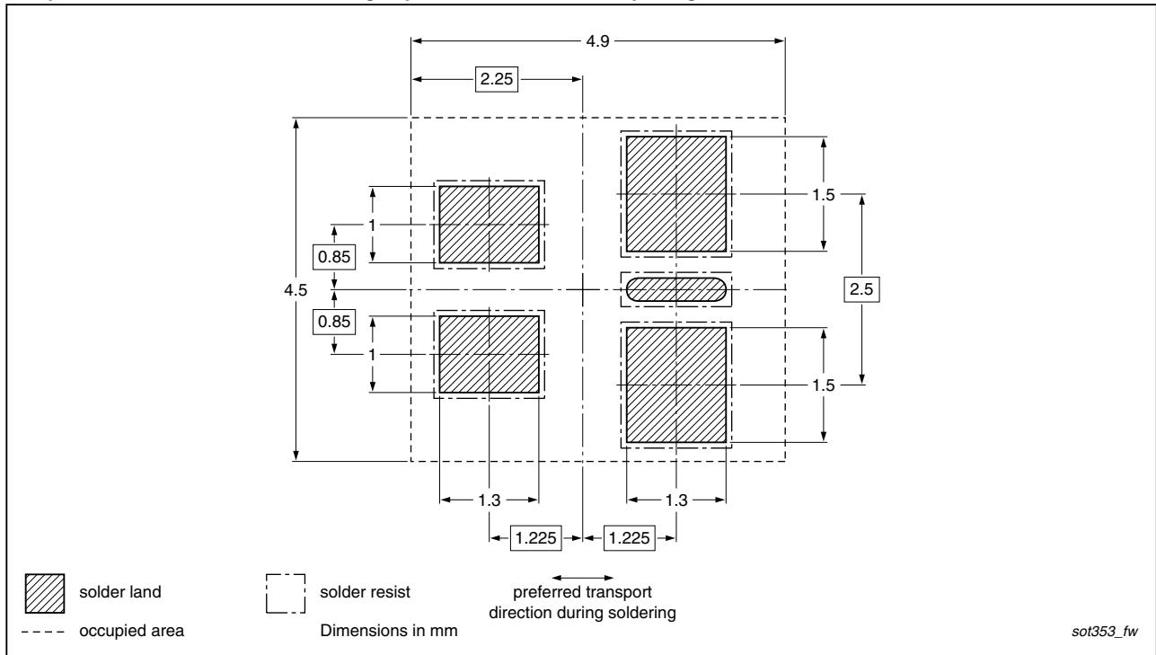
Footprint information for wave soldering of plastic surface-mounted package; 5 leads
