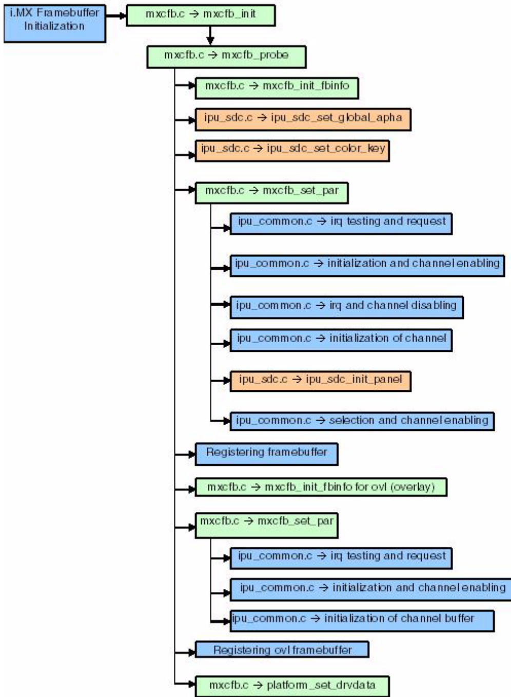
Figure 22. mxafb.c Flow Chart
