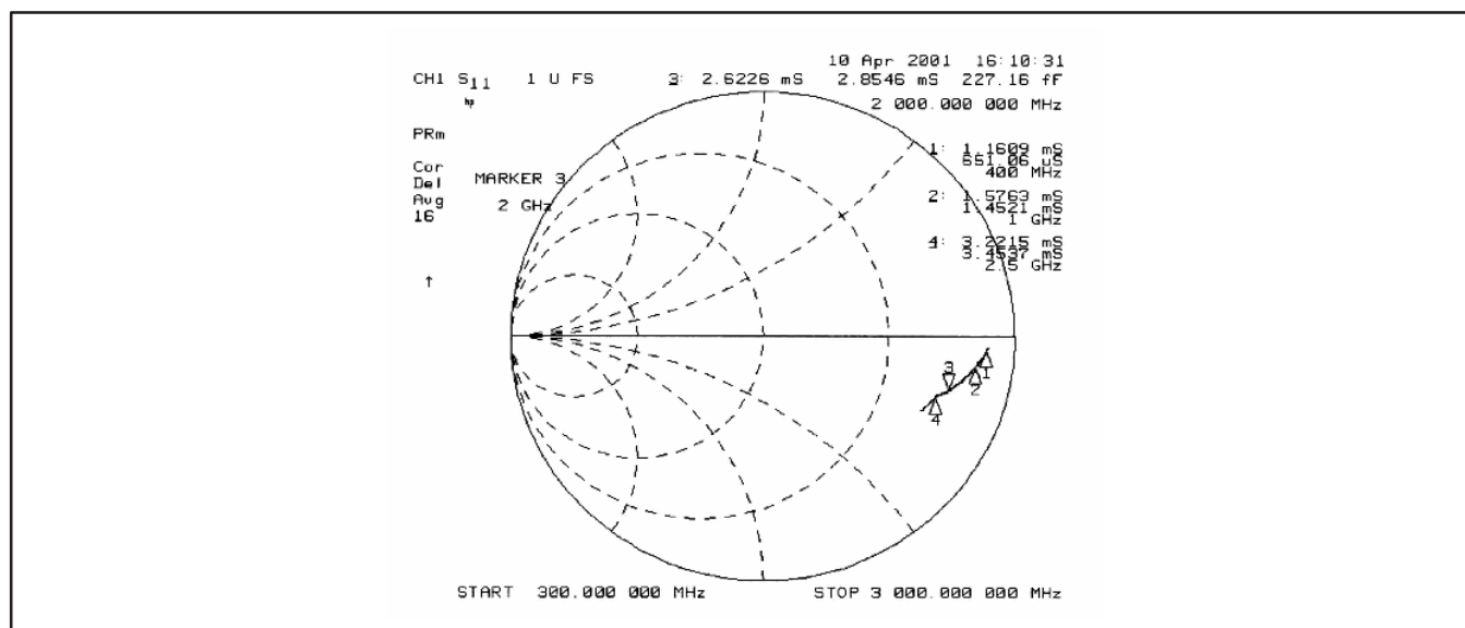
Figure 15. Typical RF/Main input impedance, V_{DD} = 3 V.
