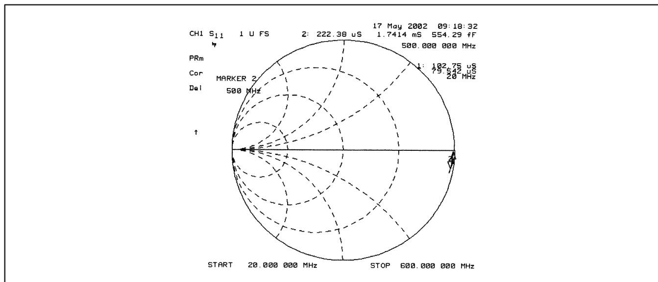
Figure 19. Typical IF/Aux input impedance, V_{DD} = 3 V.
