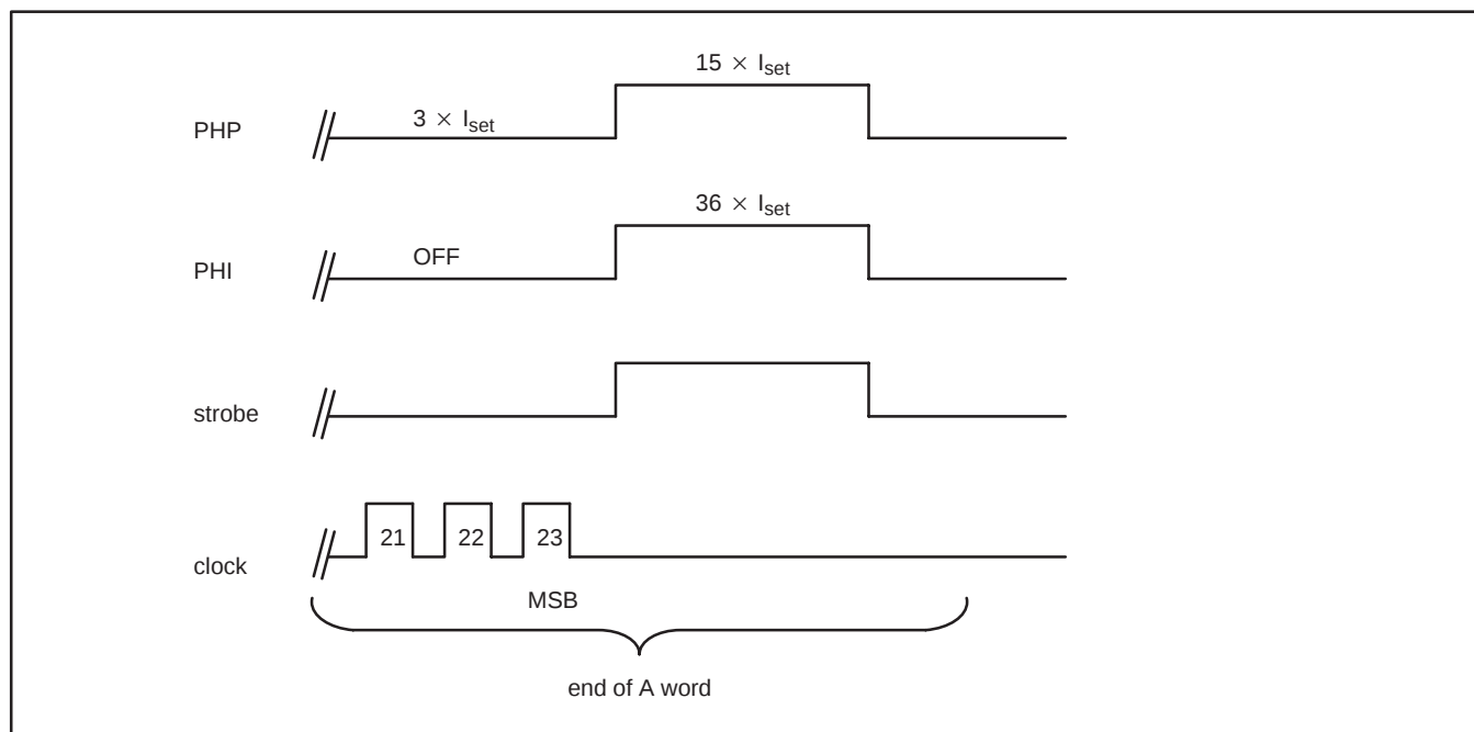
Figure 13. Pump currents related to the strobe pulse.
