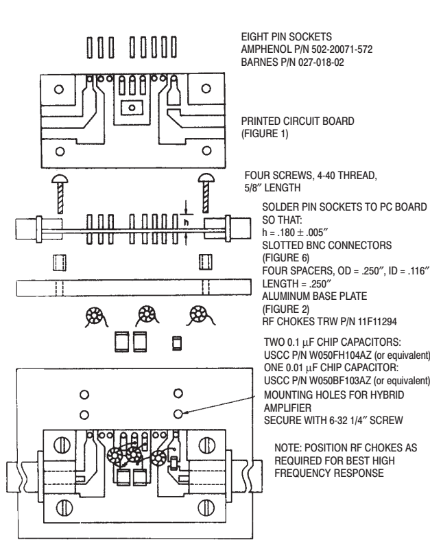
Figure 7. CA2820 Test Fixture Assembly (Case 714F-01)
