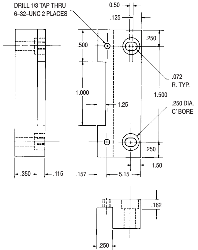
Figure 2. Heatsink Base Plate Construction for Hybrid Amplifier Test Fixture
