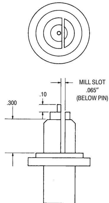
Figure 3. Adapter for Hermetic Package to Standard Hybrid Amplifier Test Fixtures
