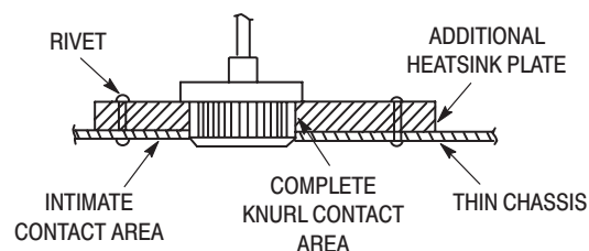
Thin-Chassis Mounting
