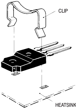
15c. Clip-Mounted Fully Isolated Package
