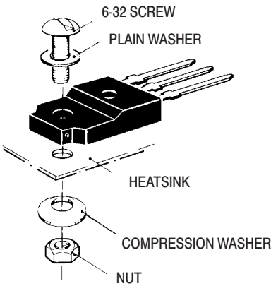
15b. Screw-Mounted Fully Isolated Package
