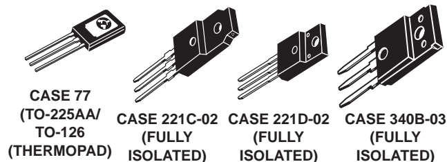
Figure 13. Plastic Body-Mount Packages
