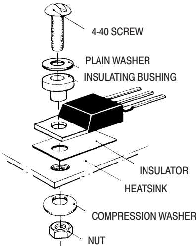
15a. Screw-Mounted TO-220
