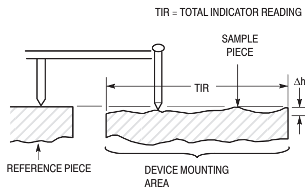
Figure 2. Surface Flatness Measurement
