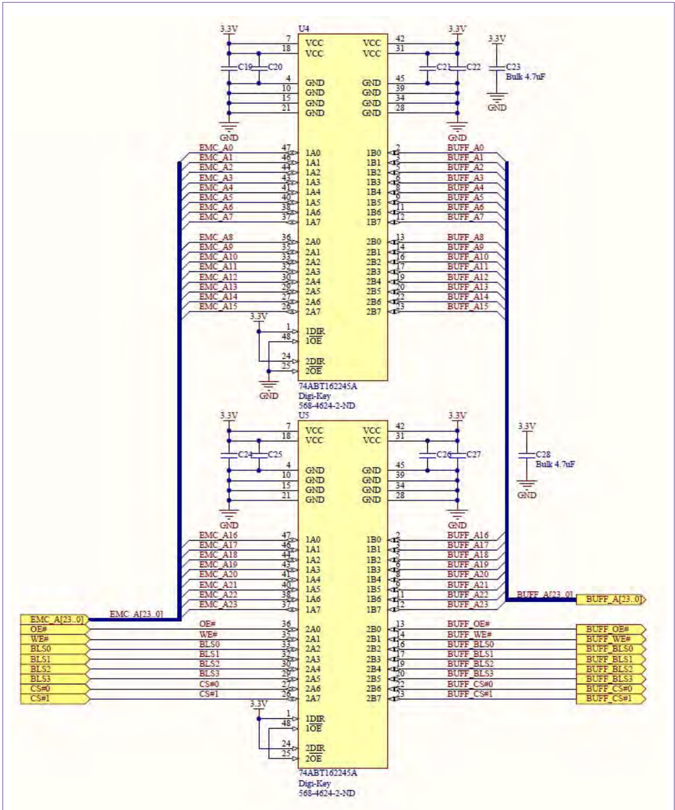
Fig 7. Address[23:0] buffering, static control buffering
