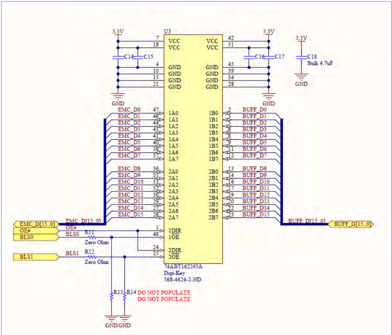
Fig 6. Data[15:0] buffering, BLS[1:0] control output enable
