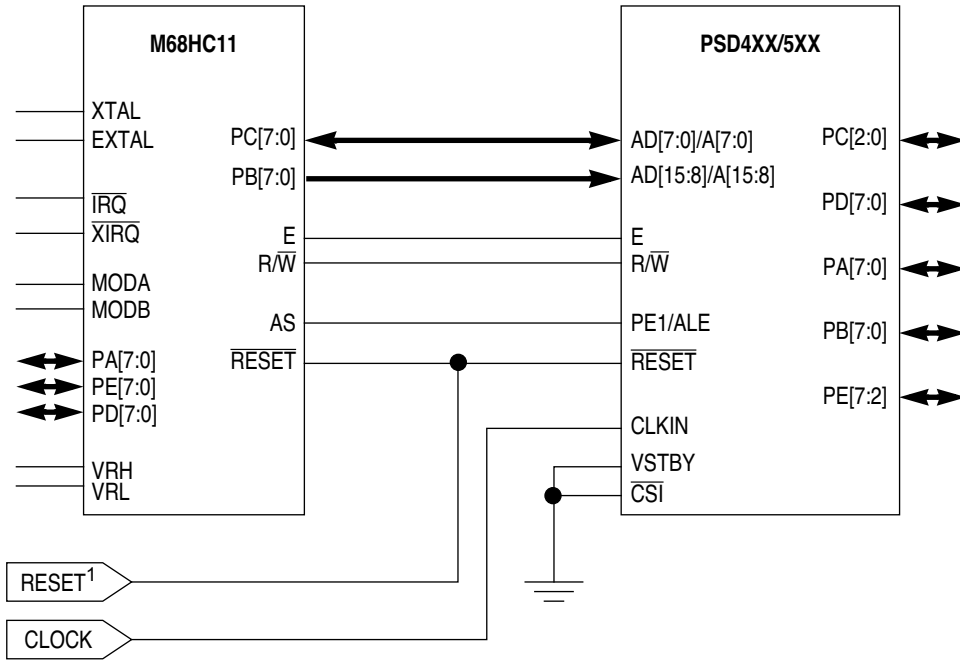
Figure 2 Typical M68HC11 and PSD4XX/5XX System
