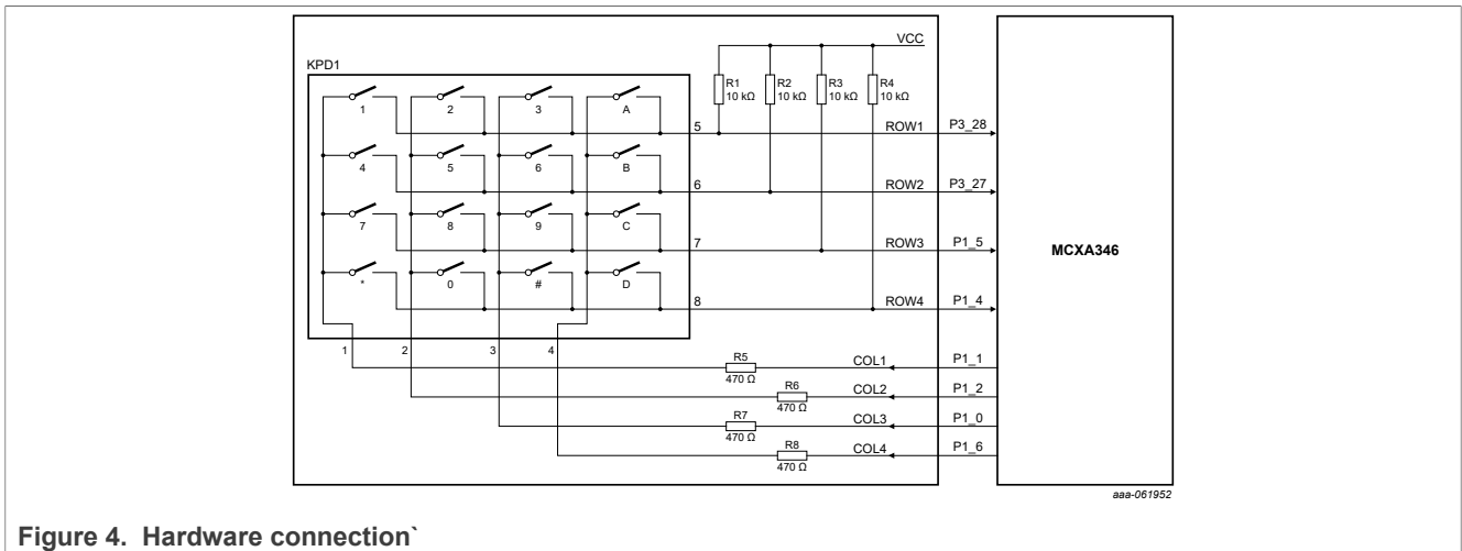
Figure 4. Hardware connection`
