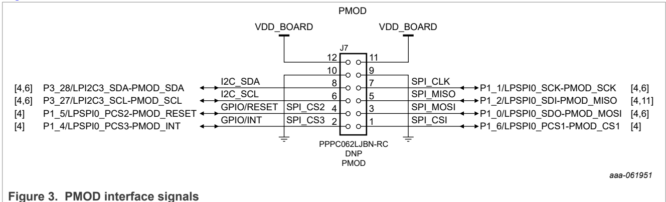
Figure 3. PMOD interface signals
