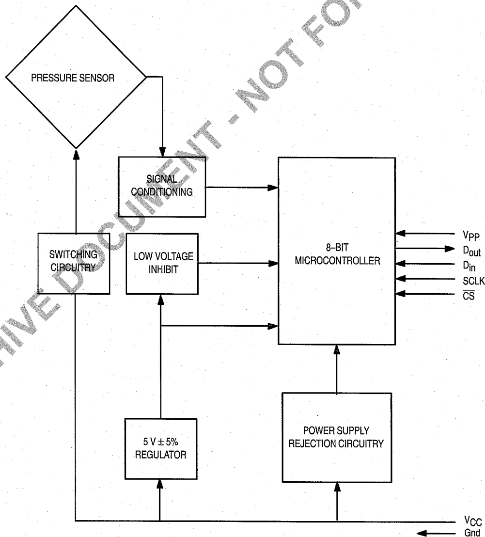
Figure 1. Smart Sensing Block Diagram
