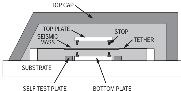
Figure 8. Accelerometer Cross Section
