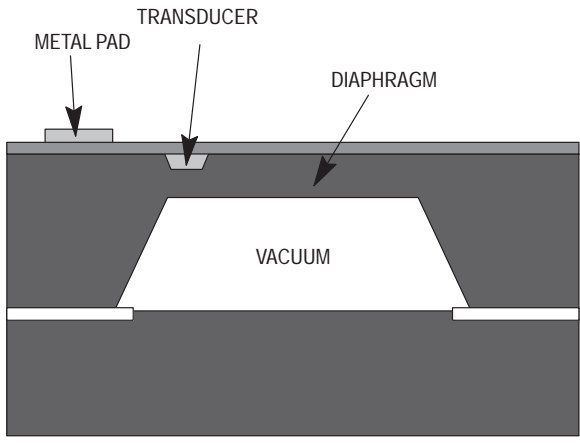
Figure 1. Pressure Sensor Cross Section
