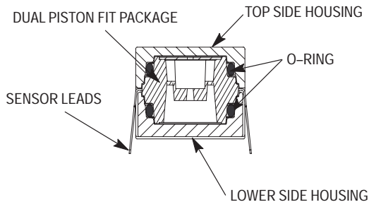
Figure 3. Dual Piston Fit Custom Housing Cross Section
