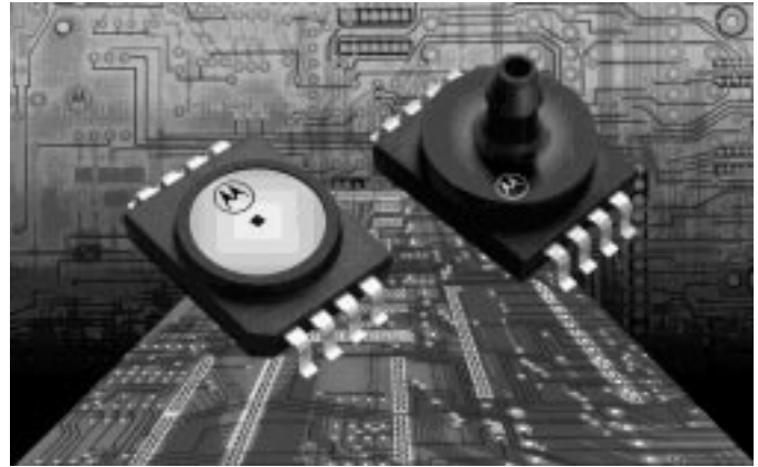
Figure 6. Piston Fit Packages Top Piston Fit (l) & Top Piston Fit with Stove Pipe Port (r)
