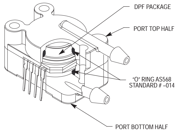
Figure 2. Dual Piston Fit Package Custom Housing
