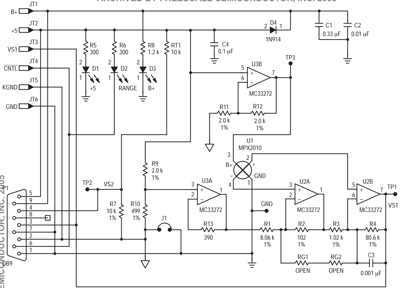
Figure 2. Schematic
