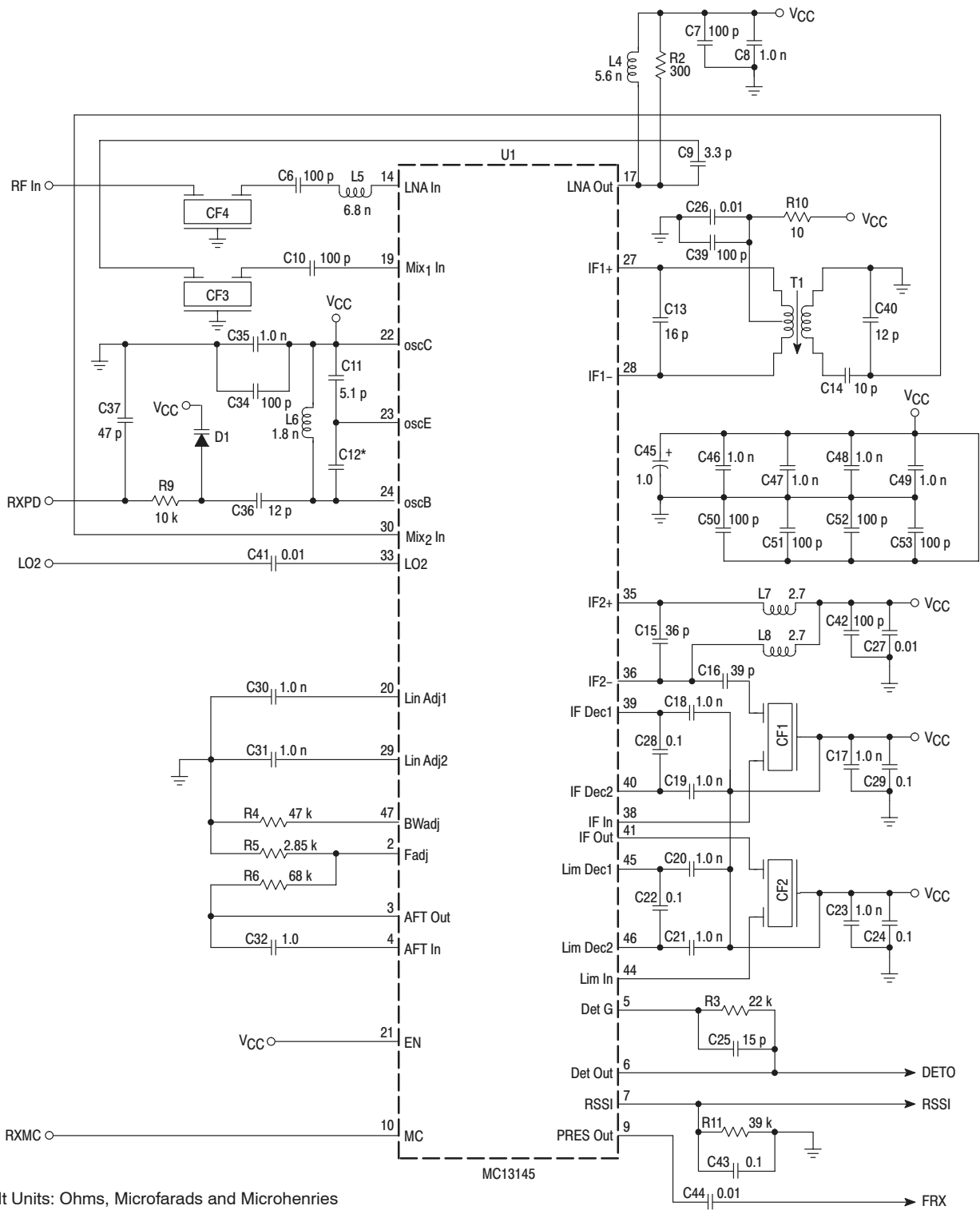
Figure 5. RF Receiver
