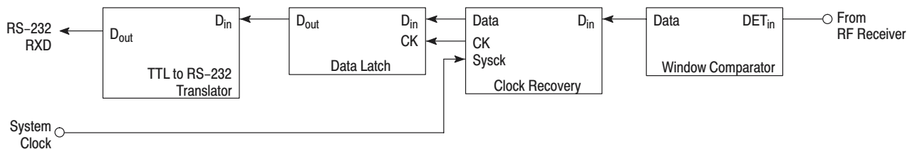
Figure 8. RS-232 Receiver
