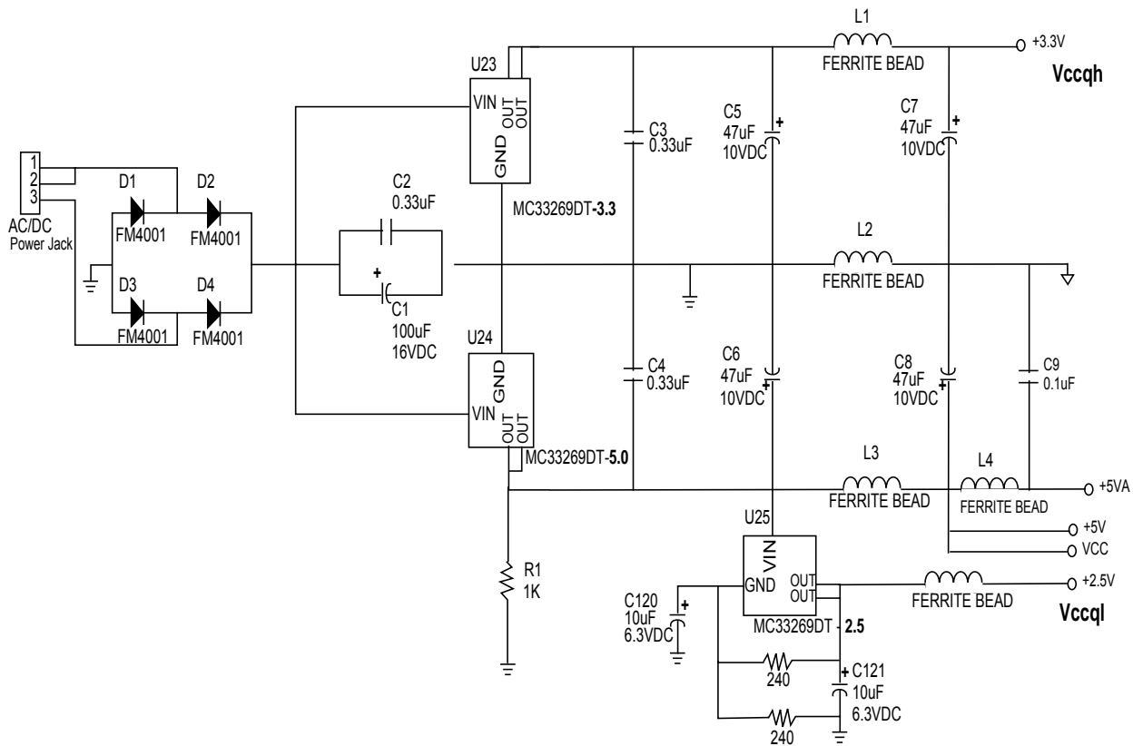
Figure 1. DSP56307 Power Supply Circuit Example
