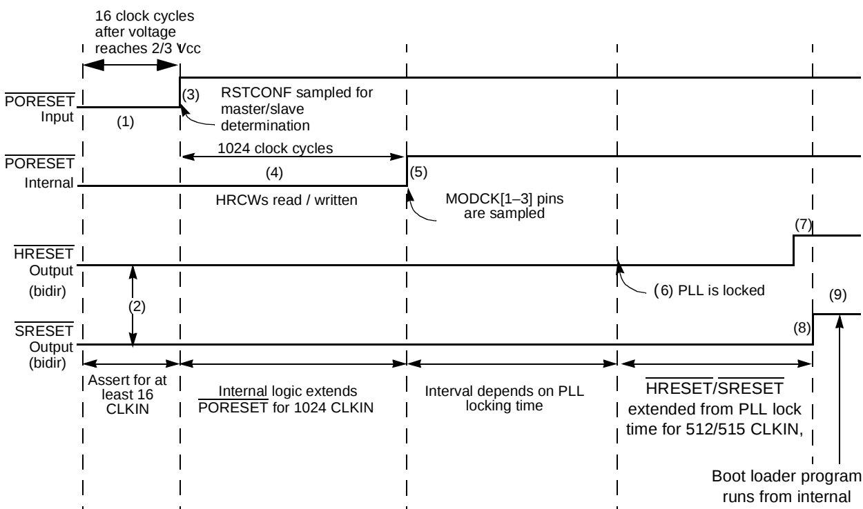
Figure 1. Timing Diagram for MSC8101 Power-On Reset Using Hardware Reset Configuration
