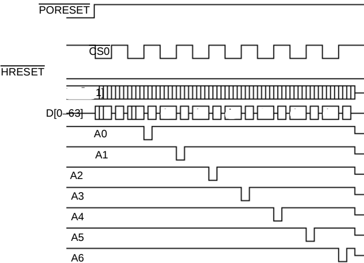
Figure 2. Power-On Reset With Multiple MSC8101 Devices
