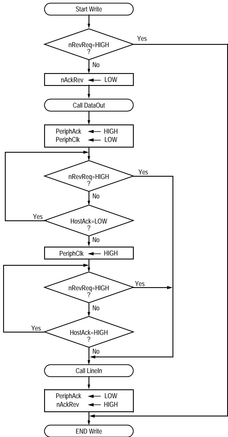
Figure 7. ECP Write Routine Flowchart
