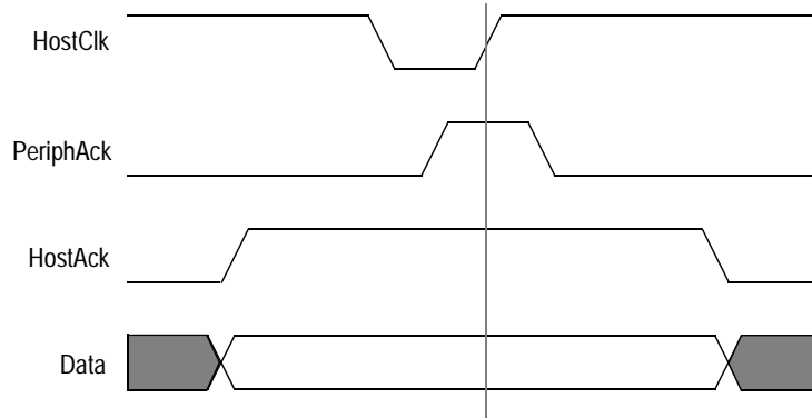
Figure 1. ECP Forward Data Cycle
