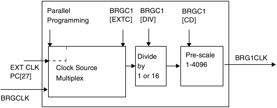
Figure 2. Baud-Rate Generator
