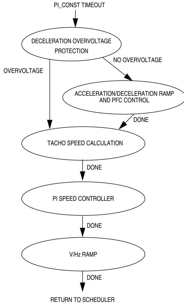
Figure 11. State Diagram — PI_CONST Timeout
