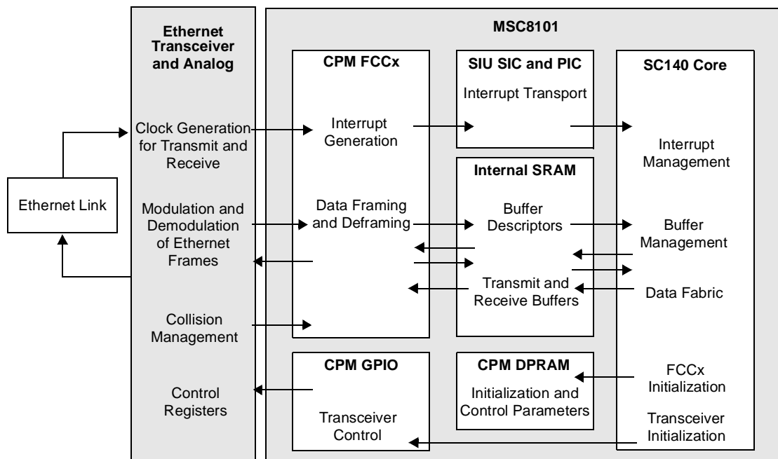
Figure 2. Control and Data Paths
