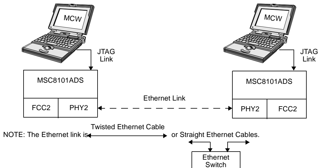
Figure 3. Set-up Using Two MSC8101ADS Boards
