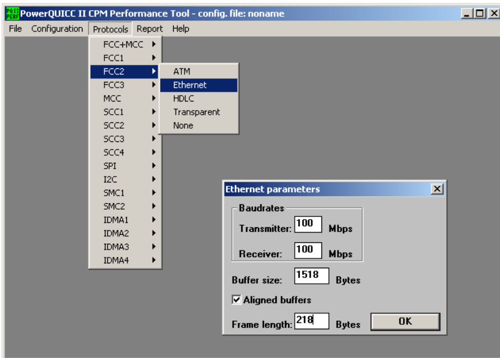
Figure 8. CPM Performance Tool, Screen 3
