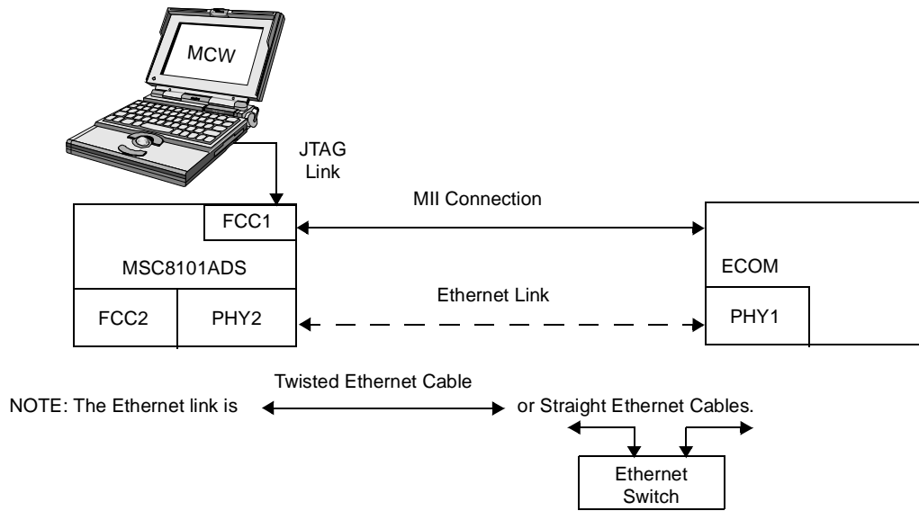
Figure 4. Set-up Using an MSC8101ADS and an ECOM Board
