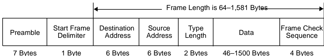
Figure 1. Ethernet Frame Format
