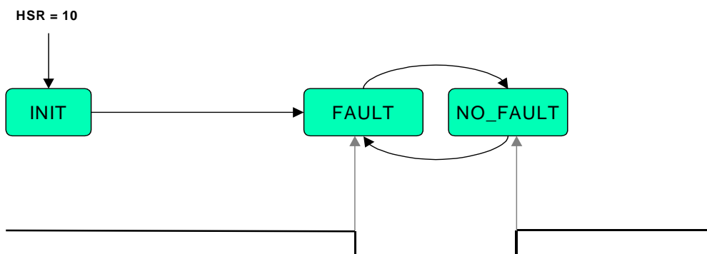
Figure 13. 3Sin3_fault timing
