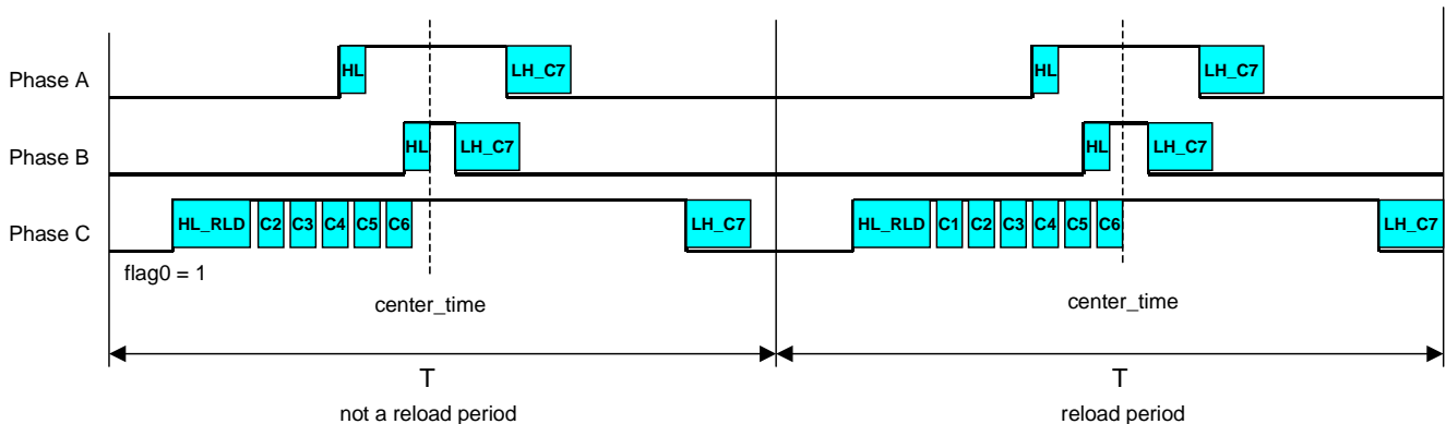
Figure 3. 3Sin3 timing
