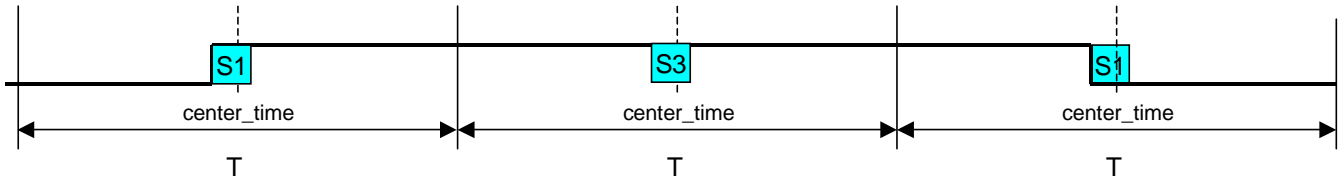
Figure 10. DcMxor_res timing
