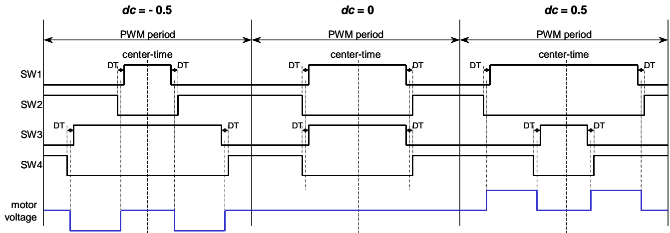
Figure 2. Unipolar switching
