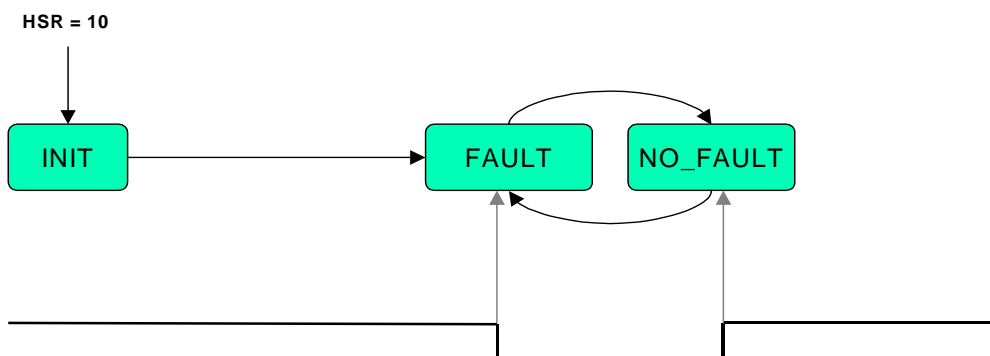
Figure 12. DCmXor_fault timing
