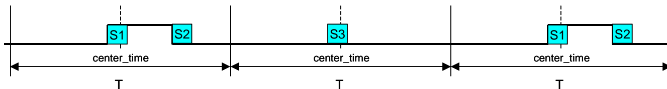
Figure 7. DCmXor_sync timing
