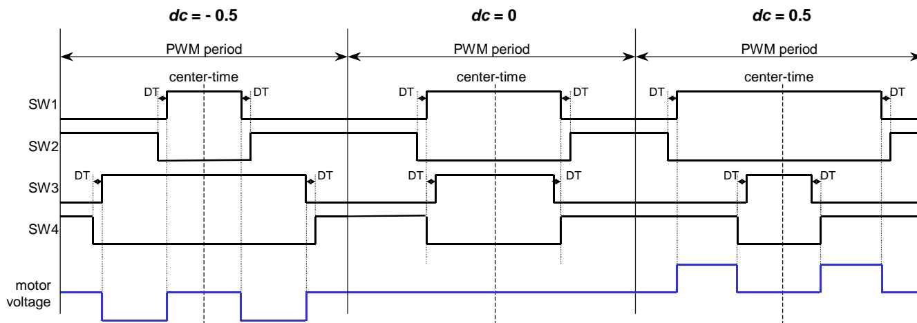
Figure 3. Unipolar switching
