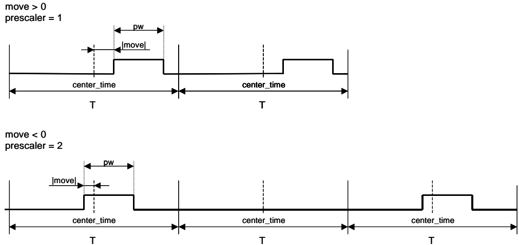
Figure 7. Synchronization signal adjustment examples
