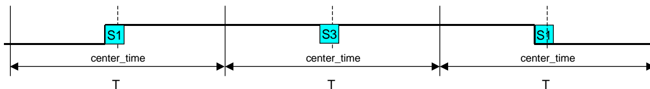
Figure 11. DCmDtXor_res timing
