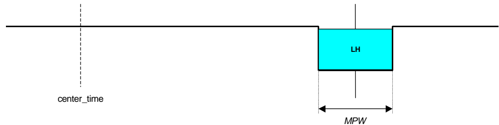
Figure 6. Timing of the worst case
