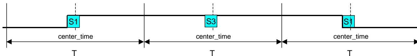
Figure 12. svmStd3_res timing
