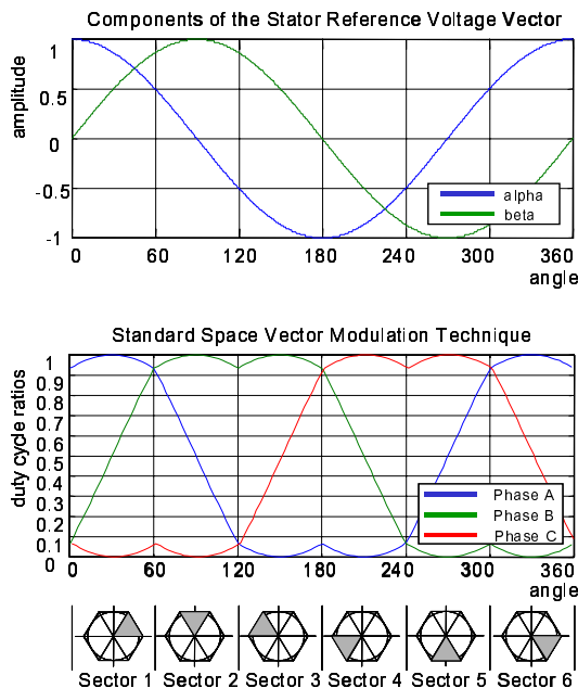
Figure 2. Standard Space Vector Modulation – 3 outputs version Technique
