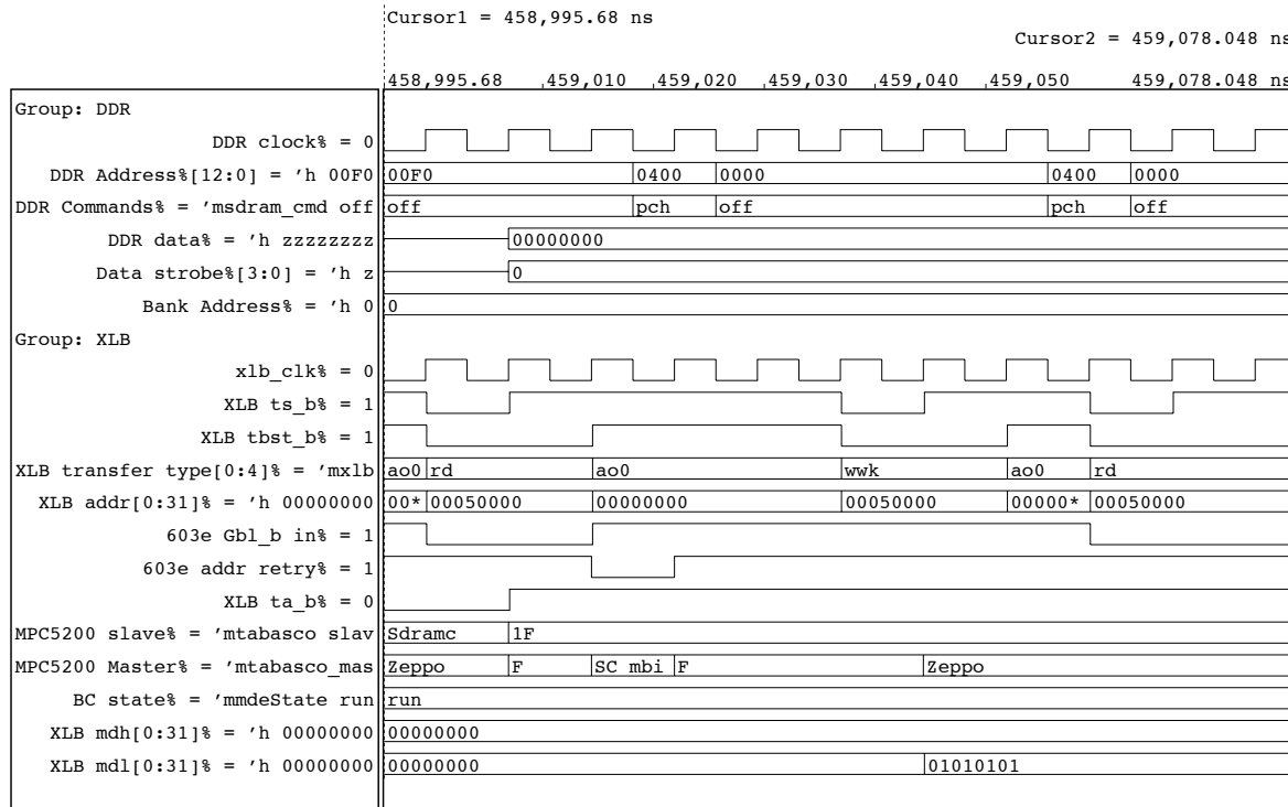
Figure 5. Address Retry
