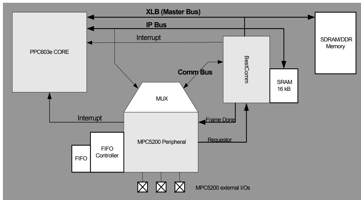
Figure 2. BestComm's Architecture
